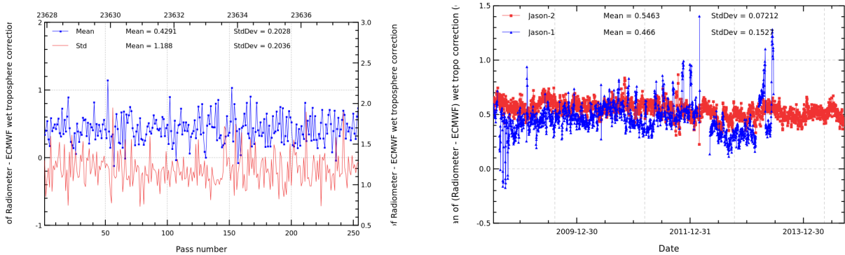
FIGURE 11 – Pass monitoring of wet troposphere differences between radiometer and ECMWF model for Jason-2 cycle 228 (left) and daily monitoring of wet troposphere differences between radiometer and ECMWF model (right).
