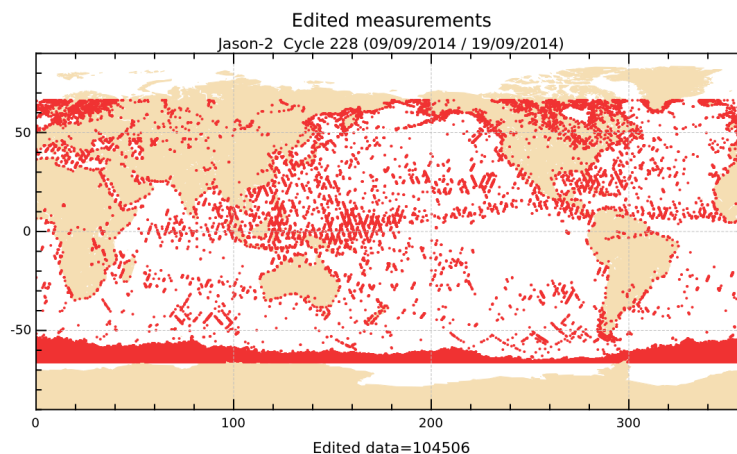
FIGURE 2 – Edited measurements for cycle 228.
