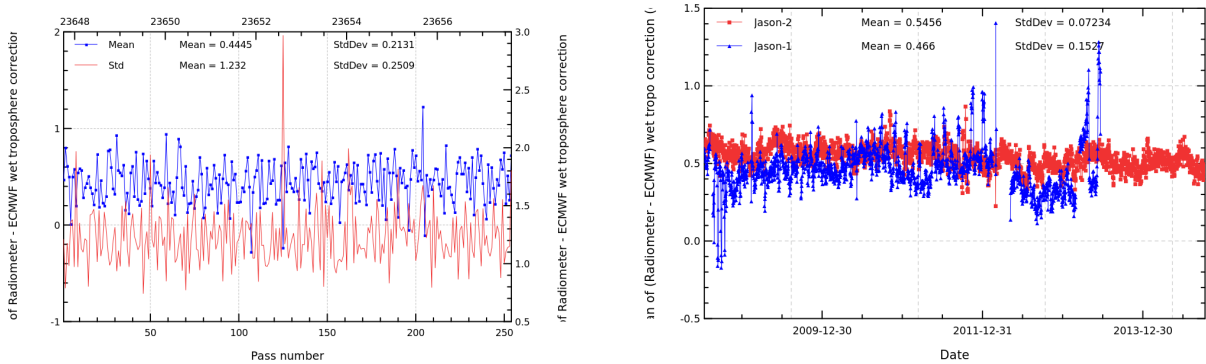
FIGURE 11 – Pass monitoring of wet troposphere differences between radiometer and ECMWF model for Jason-2 cycle 230 (left) and daily monitoring of wet troposphere differences between radiometer and ECMWF model (right).
