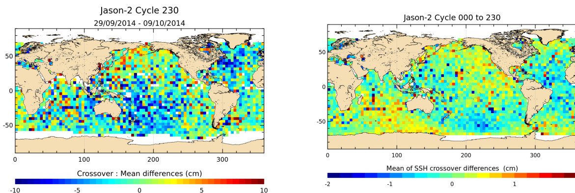
FIGURE 12 – Mean SSH at crossovers for cycle 230 (left) and over the whole Jason-2 period (right).
