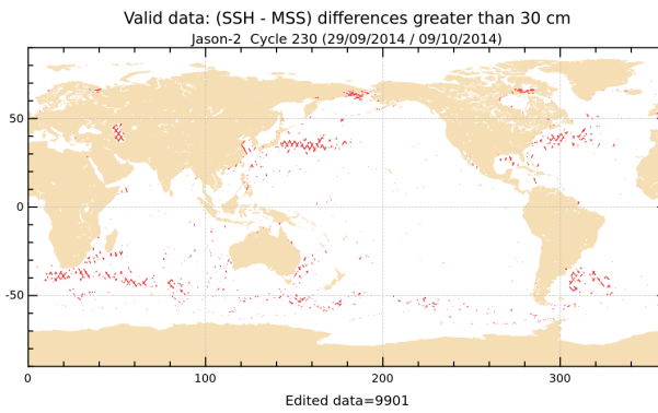
FIGURE 18 – Differences higher than a 30 cm threshold for cycle 230.
