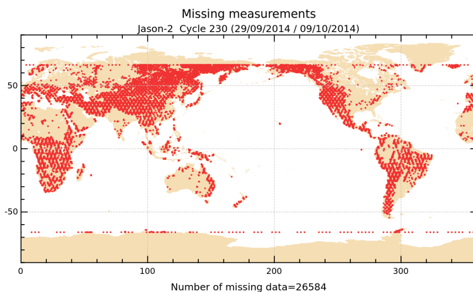
FIGURE 1 – Missing measurements for cycle 230.
