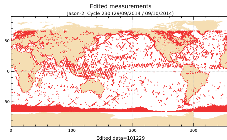
FIGURE 2 – Edited measurements for cycle 230.
