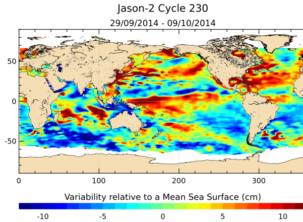
FIGURE 17 – Sea level anomaly relative to MSS for cycle 230.
