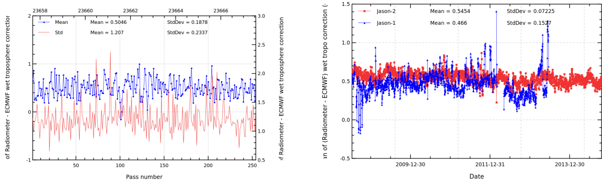
FIGURE 11 – Pass monitoring of wet troposphere differences between radiometer and ECMWF model for Jason-2 cycle 231 (left) and daily monitoring of wet troposphere differences between radiometer and ECMWF model (right).
