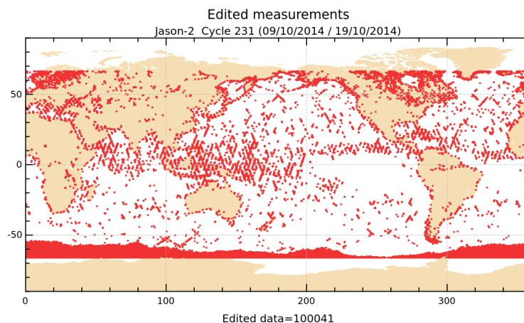
FIGURE 2 – Edited measurements for cycle 231.
