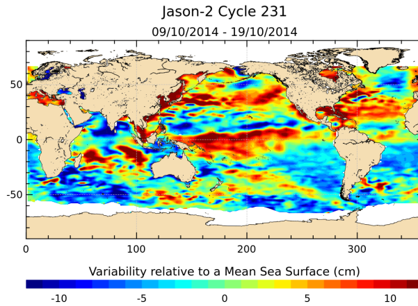
FIGURE 17 – Sea level anomaly relative to MSS for cycle 231.
