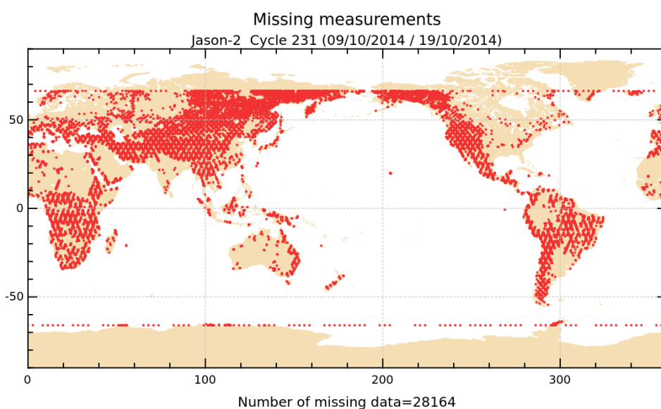
FIGURE 1 – Missing measurements for cycle 231.
