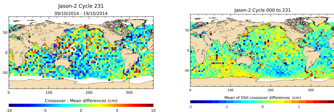
FIGURE 12 – Mean SSH at crossovers for cycle 231 (left) and over the whole Jason-2 period (right).
