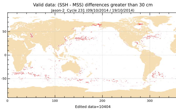
FIGURE 18 – Differences higher than a 30 cm threshold for cycle 231.
