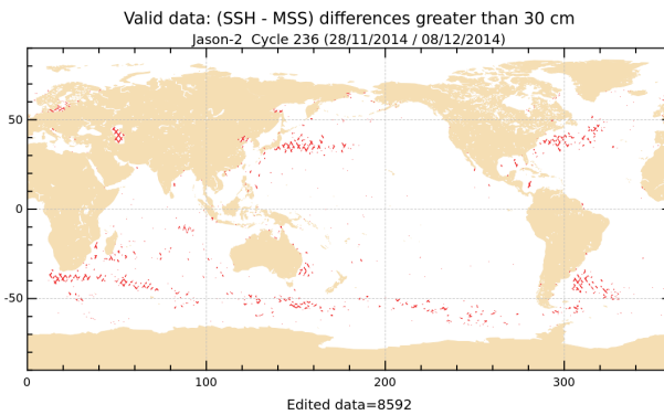
FIGURE 19 – Differences higher than a 30 cm threshold for cycle 236.
