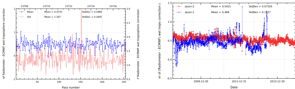
FIGURE 12 – Pass monitoring of wet troposphere differences between radiometer and ECMWF model for Jason-2 cycle 236 (left) and daily monitoring of wet troposphere differences between radiometer and ECMWF model (right).
