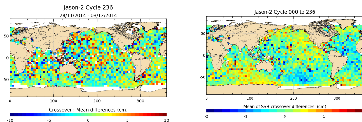
FIGURE 13 – Mean SSH at crossovers for cycle 236 (left) and over the whole Jason-2 period (right).
