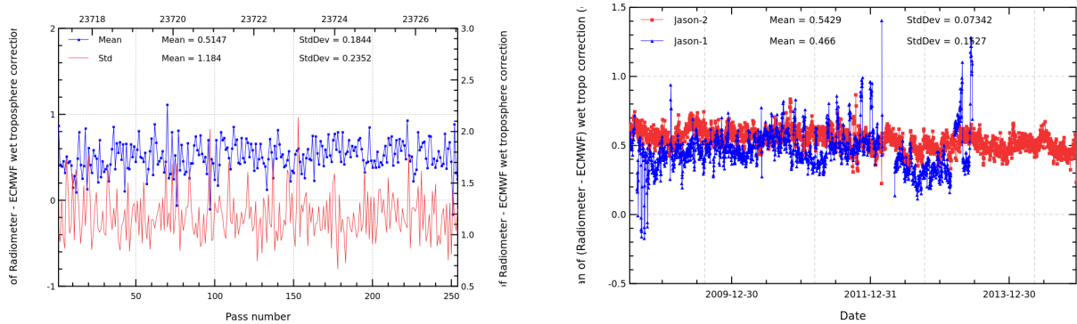
FIGURE 11 – Pass monitoring of wet troposphere differences between radiometer and ECMWF model for Jason-2 cycle 237 (left) and daily monitoring of wet troposphere differences between radiometer and ECMWF model (right).
