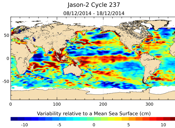
FIGURE 17 – Sea level anomaly relative to MSS for cycle 237.
