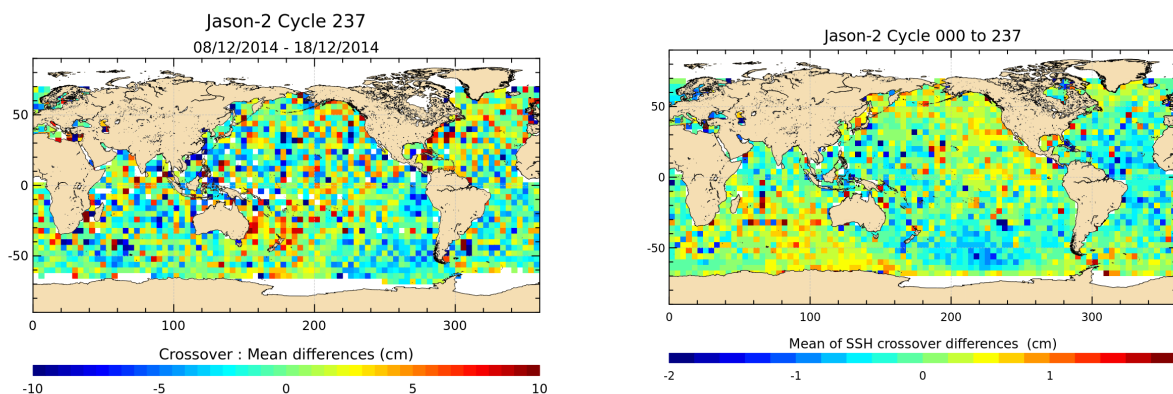
FIGURE 12 – Mean SSH at crossovers for cycle 237 (left) and over the whole Jason-2 period (right).
