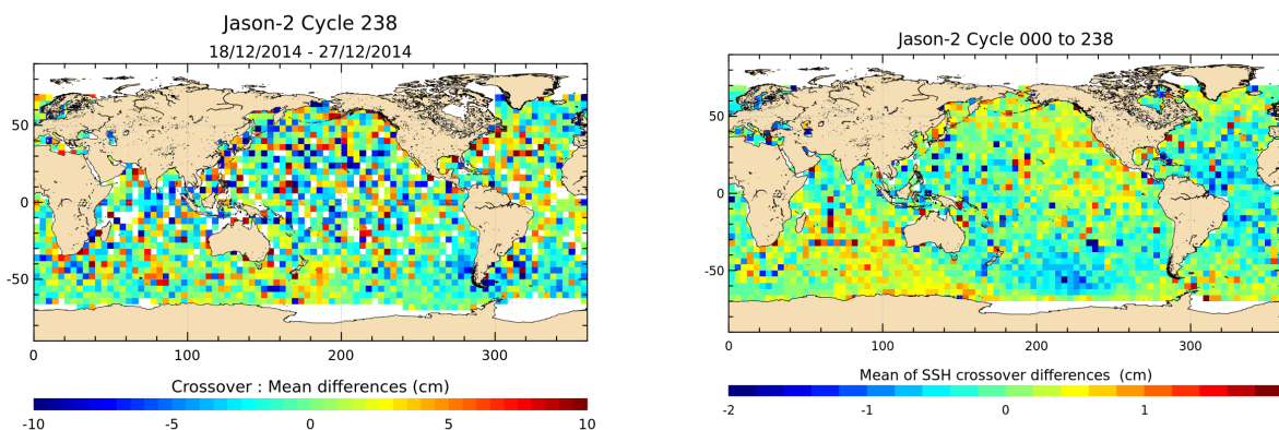
FIGURE 12 – Mean SSH at crossovers for cycle 238 (left) and over the whole Jason-2 period (right).
