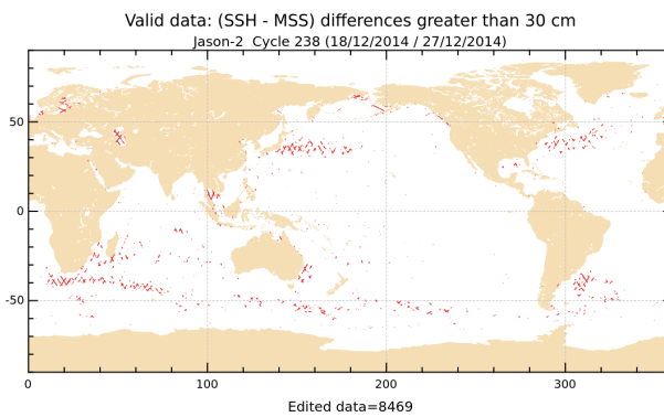
FIGURE 18 – Differences higher than a 30 cm threshold for cycle 238.
