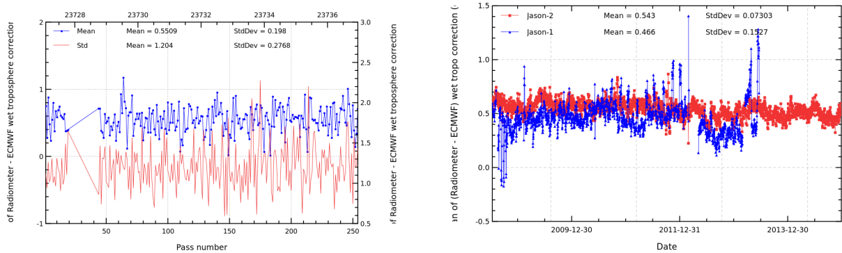
FIGURE 11 – Pass monitoring of wet troposphere differences between radiometer and ECMWF model for Jason-2 cycle 238 (left) and daily monitoring of wet troposphere differences between radiometer and ECMWF model (right).
