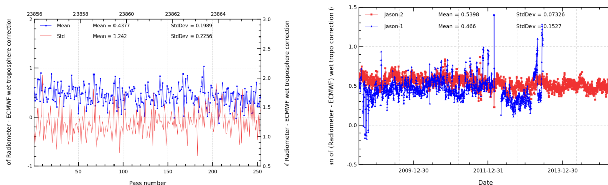
FIGURE 11 – Pass monitoring of wet troposphere differences between radiometer and ECMWF model for Jason-2 cycle 251 (left) and daily monitoring of wet troposphere differences between radiometer and ECMWF model (right).
