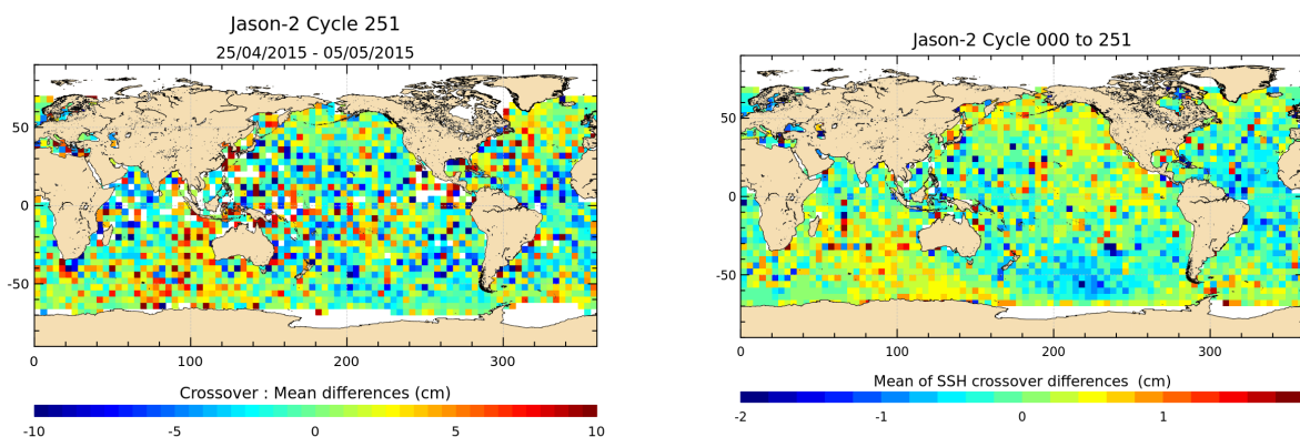
FIGURE 12 – Mean SSH at crossovers for cycle 251 (left) and over the whole Jason-2 period (right).
