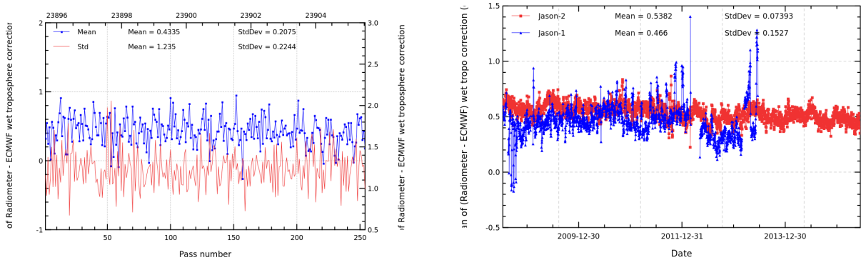
FIGURE 11 – Pass monitoring of wet troposphere differences between radiometer and ECMWF model for Jason-2 cycle 255 (left) and daily monitoring of wet troposphere differences between radiometer and ECMWF model (right).
