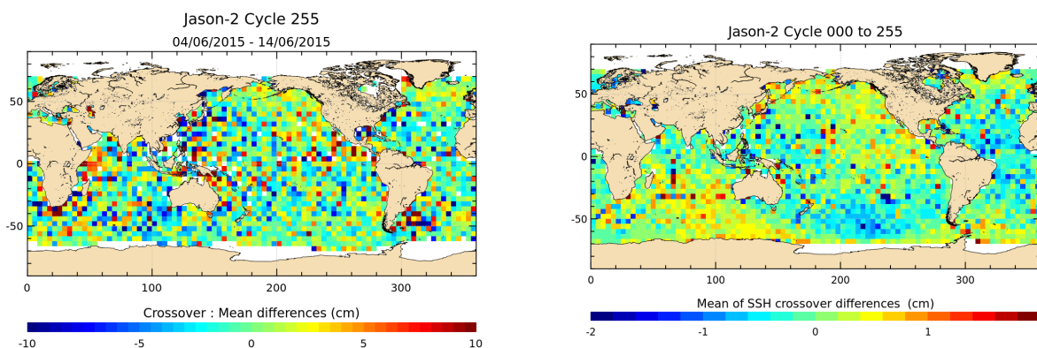
FIGURE 12 – Mean SSH at crossovers for cycle 255 (left) and over the whole Jason-2 period (right).
