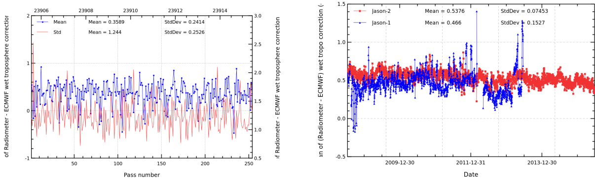
FIGURE 11 – Pass monitoring of wet troposphere differences between radiometer and ECMWF model for Jason-2 cycle 256 (left) and daily monitoring of wet troposphere differences between radiometer and ECMWF model (right).
