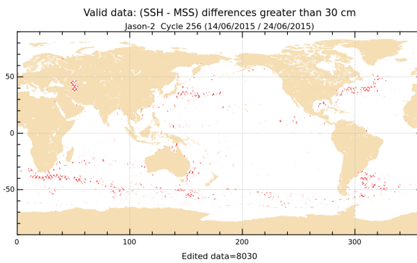
FIGURE 18 – Differences higher than a 30 cm threshold for cycle 256.
