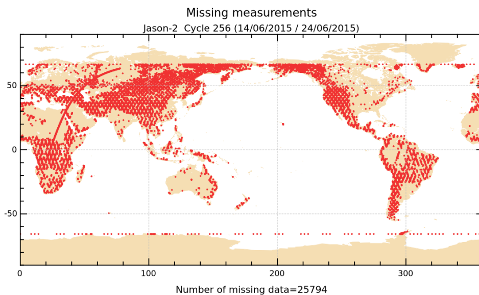
FIGURE 1 – Missing measurements for cycle 256.
