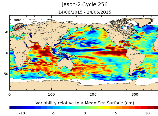
FIGURE 17 – Sea level anomaly relative to MSS for cycle 256.
