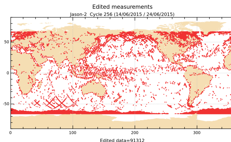
FIGURE 2 – Edited measurements for cycle 256.
