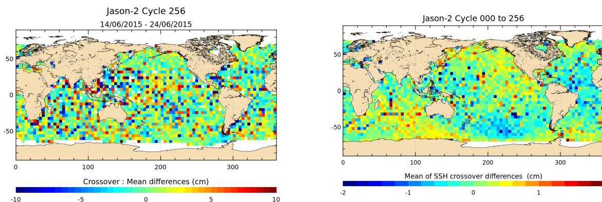
FIGURE 12 – Mean SSH at crossovers for cycle 256 (left) and over the whole Jason-2 period (right).
