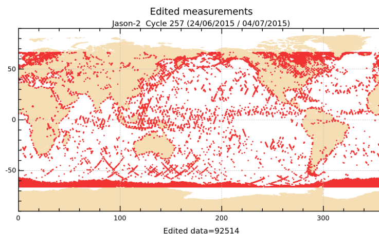
FIGURE 2 – Edited measurements for cycle 257.
