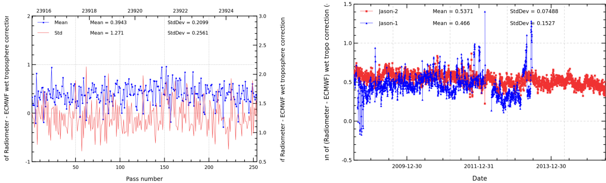
FIGURE 11 – Pass monitoring of wet troposphere differences between radiometer and ECMWF model for Jason-2 cycle 257 (left) and daily monitoring of wet troposphere differences between radiometer and ECMWF model (right).
