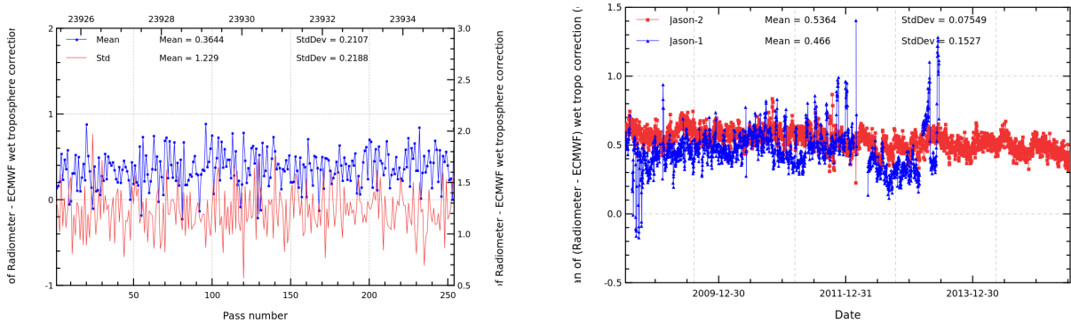
FIGURE 11 – Pass monitoring of wet troposphere differences between radiometer and ECMWF model for Jason-2 cycle 258 (left) and daily monitoring of wet troposphere differences between radiometer and ECMWF model (right).
