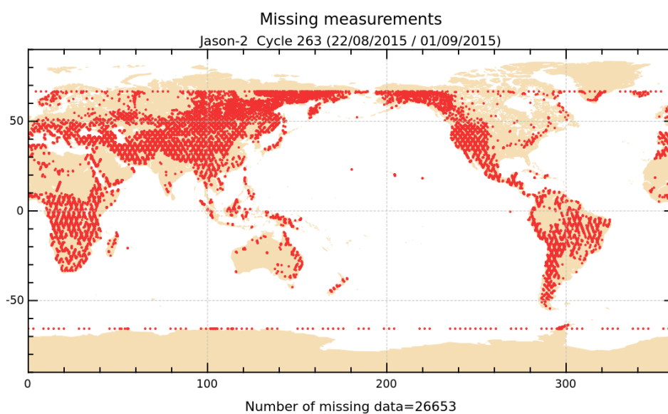
FIGURE 1 – Missing measurements for cycle 263.
