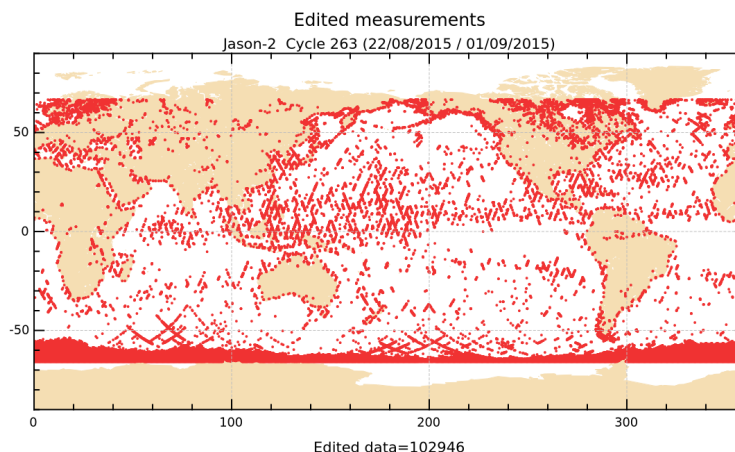
FIGURE 2 – Edited measurements for cycle 263.
