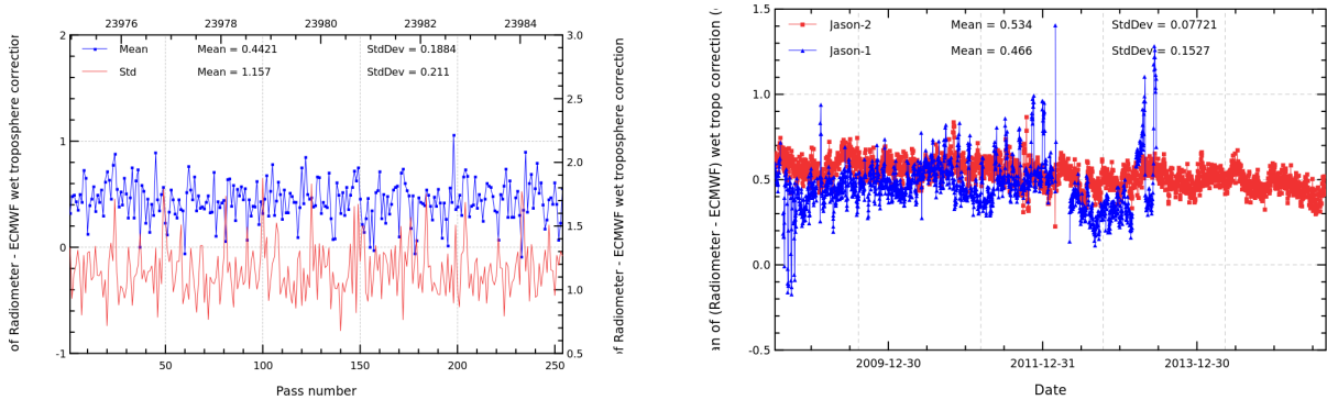
FIGURE 11 – Pass monitoring of wet troposphere differences between radiometer and ECMWF model for Jason-2 cycle 263 (left) and daily monitoring of wet troposphere differences between radiometer and ECMWF model (right).
