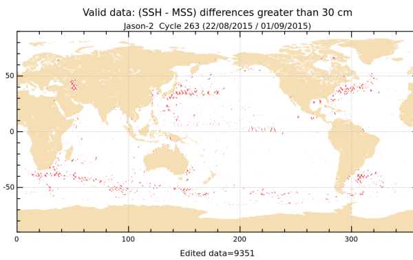
FIGURE 18 – Differences higher than a 30 cm threshold for cycle 263.
