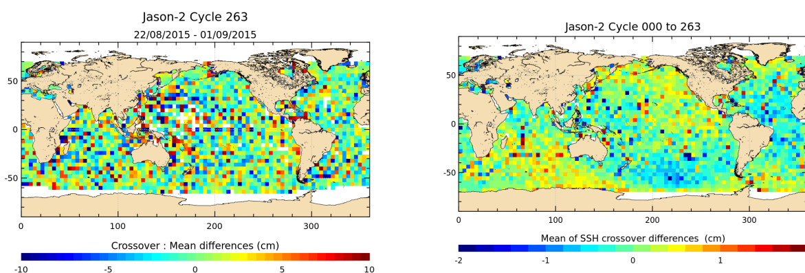
FIGURE 12 – Mean SSH at crossovers for cycle 263 (left) and over the whole Jason-2 period (right).
