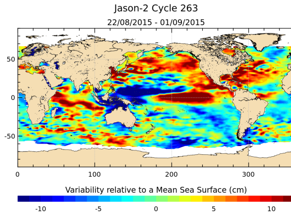
FIGURE 17 – Sea level anomaly relative to MSS for cycle 263.
