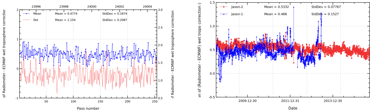
FIGURE 11 – Pass monitoring of wet troposphere differences between radiometer and ECMWF model for Jason-2 cycle 265 (left) and daily monitoring of wet troposphere differences between radiometer and ECMWF model (right).
