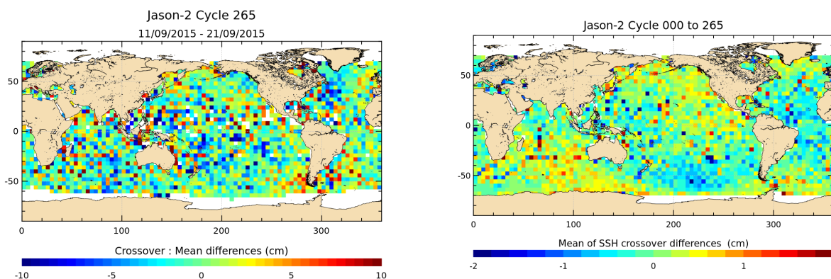
FIGURE 13 – Mean SSH at crossovers for cycle 265 (left) and over the whole Jason-2 period (right).
