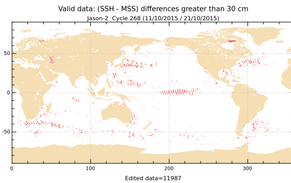
FIGURE 18 – Differences higher than a 30 cm threshold for cycle 268.
