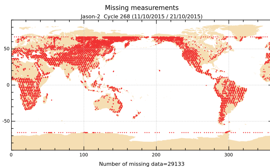
FIGURE 1 – Missing measurements for cycle 268.
