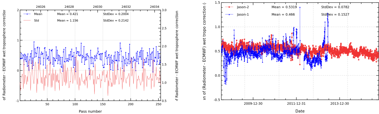
FIGURE 11 – Pass monitoring of wet troposphere differences between radiometer and ECMWF model for Jason-2 cycle 268 (left) and daily monitoring of wet troposphere differences between radiometer and ECMWF model (right).
