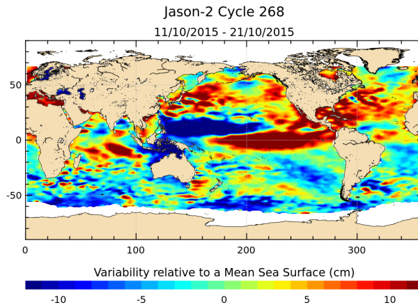
FIGURE 17 – Sea level anomaly relative to MSS for cycle 268.
