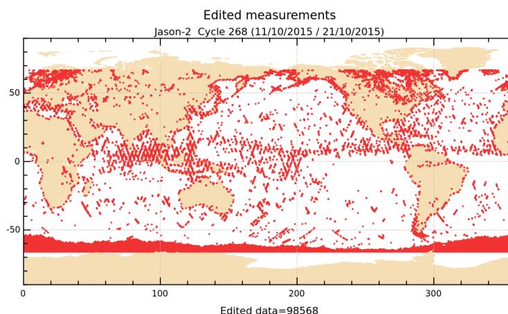
FIGURE 2 – Edited measurements for cycle 268.
