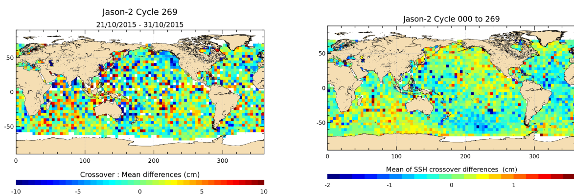
FIGURE 12 – Mean SSH at crossovers for cycle 269 (left) and over the whole Jason-2 period (right).
