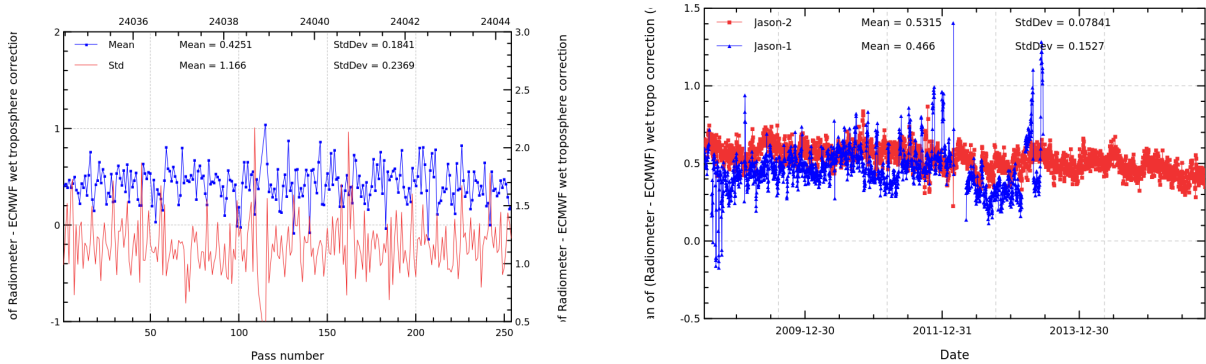
FIGURE 11 – Pass monitoring of wet troposphere differences between radiometer and ECMWF model for Jason-2 cycle 269 (left) and daily monitoring of wet troposphere differences between radiometer and ECMWF model (right).
