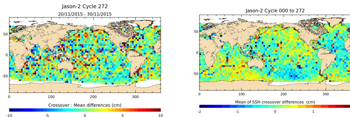
FIGURE 12 – Mean SSH at crossovers for cycle 272 (left) and over the whole Jason-2 period (right).
