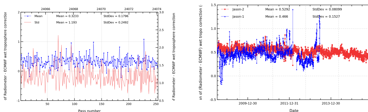
FIGURE 11 – Pass monitoring of wet troposphere differences between radiometer and ECMWF model for Jason-2 cycle 272 (left) and daily monitoring of wet troposphere differences between radiometer and ECMWF model (right).
