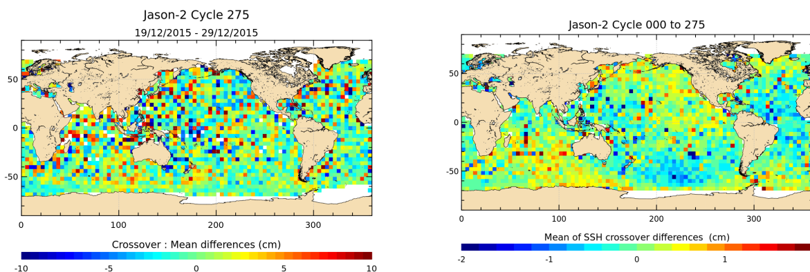
FIGURE 12 – Mean SSH at crossovers for cycle 275 (left) and over the whole Jason-2 period (right).
