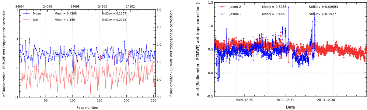
FIGURE 11 – Pass monitoring of wet troposphere differences between radiometer and ECMWF model for Jason-2 cycle 275 (left) and daily monitoring of wet troposphere differences between radiometer and ECMWF model (right).
