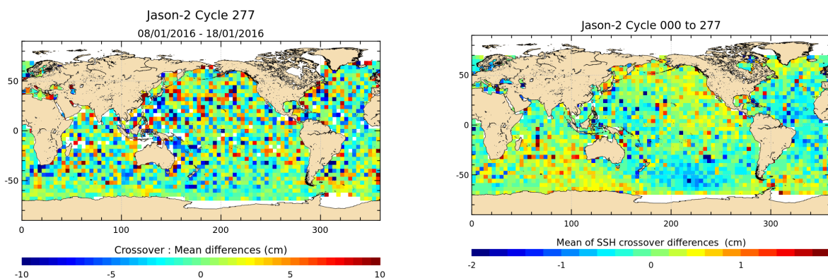
FIGURE 12 – Mean SSH at crossovers for cycle 277 (left) and over the whole Jason-2 period (right).
