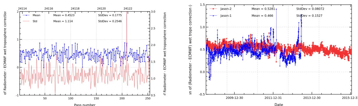
FIGURE 11 – Pass monitoring of wet troposphere differences between radiometer and ECMWF model for Jason-2 cycle 277 (left) and daily monitoring of wet troposphere differences between radiometer and ECMWF model (right).
