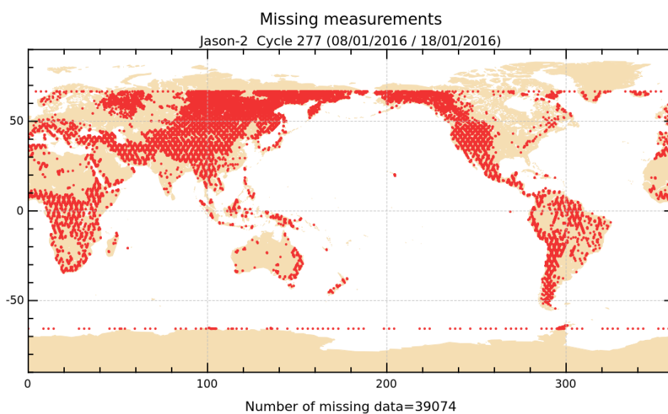
FIGURE 1 – Missing measurements for cycle 277.
