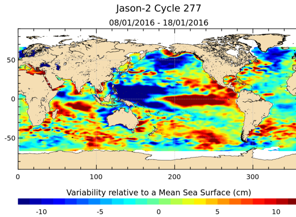
FIGURE 17 – Sea level anomaly relative to MSS for cycle 277.
