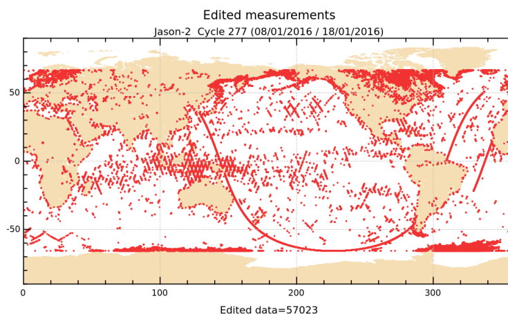
FIGURE 2 – Edited measurements for cycle 277.
