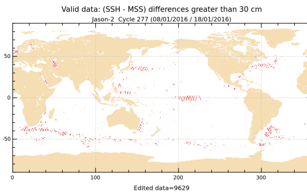
FIGURE 18 – Differences higher than a 30 cm threshold for cycle 277.
