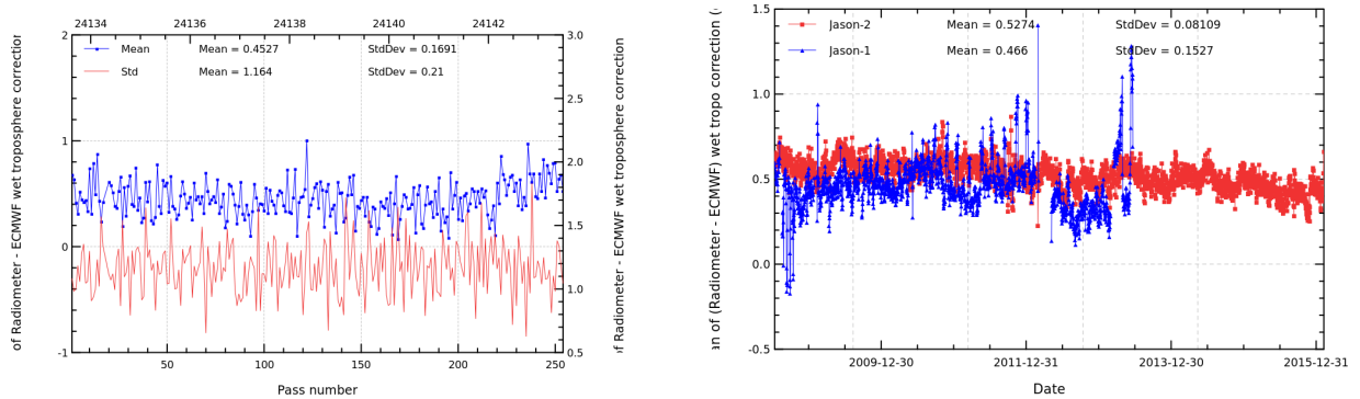
FIGURE 11 – Pass monitoring of wet troposphere differences between radiometer and ECMWF model for Jason-2 cycle 279 (left) and daily monitoring of wet troposphere differences between radiometer and ECMWF model (right).
