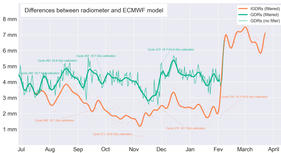
FIGURE 12 – Daily monitoring of radiometer minus ECMWF model wet troposphere difference.
