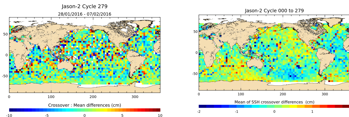
FIGURE 13 – Mean SSH at crossovers for cycle 279 (left) and over the whole Jason-2 period (right).
