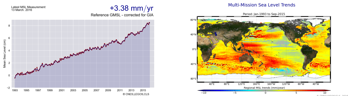
FIGURE 21 – Global (left) and regional (right) MSL trends from 1993 onwards.
