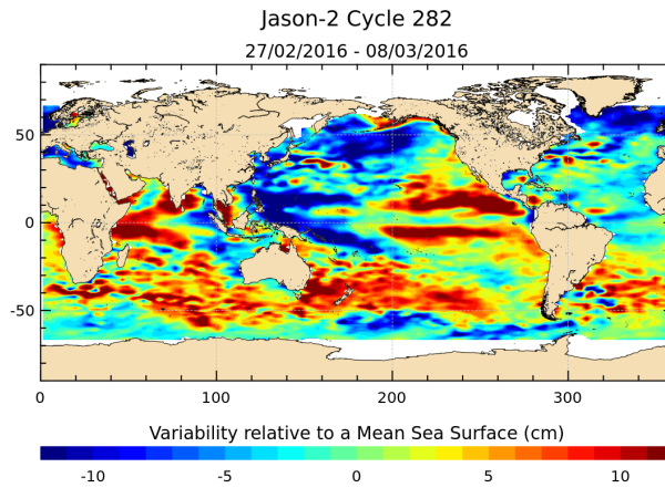
FIGURE 17 – Sea level anomaly relative to MSS for cycle 282.
