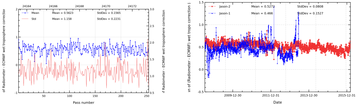
FIGURE 11 – Pass monitoring of wet troposphere differences between radiometer and ECMWF model for Jason-2 cycle 282 (left) and daily monitoring of wet troposphere differences between radiometer and ECMWF model (right).
