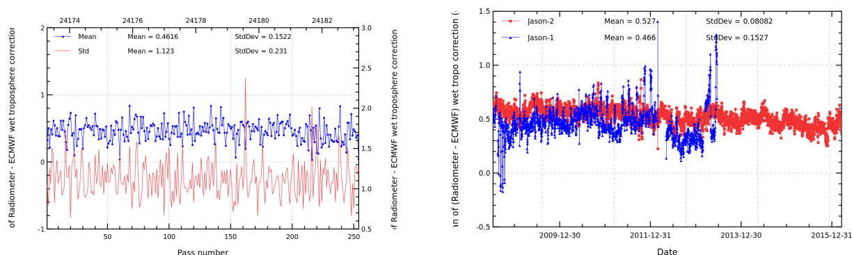
FIGURE 12 – Pass monitoring of wet troposphere differences between radiometer and ECMWF model for Jason-2 cycle 283 (left) and daily monitoring of wet troposphere differences between radiometer and ECMWF model (right).
