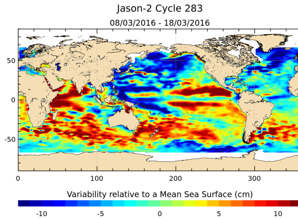
FIGURE 18 – Sea level anomaly relative to MSS for cycle 283.
