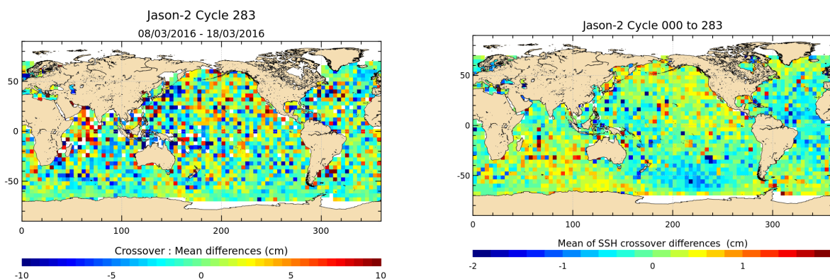
FIGURE 13 – Mean SSH at crossovers for cycle 283 (left) and over the whole Jason-2 period (right).
