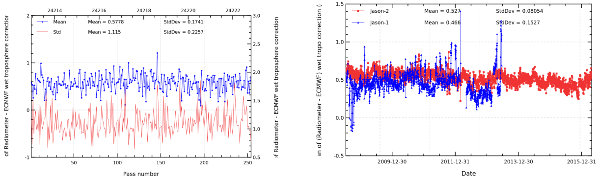
FIGURE 11 – Pass monitoring of wet troposphere differences between radiometer and ECMWF model for Jason-2 cycle 287 (left) and daily monitoring of wet troposphere differences between radiometer and ECMWF model (right).
