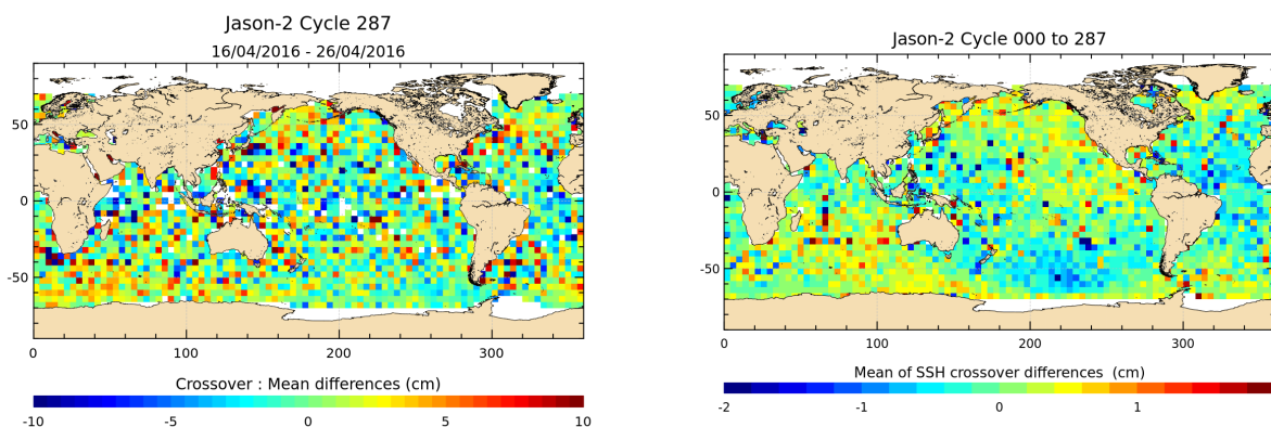
FIGURE 12 – Mean SSH at crossovers for cycle 287 (left) and over the whole Jason-2 period (right).
