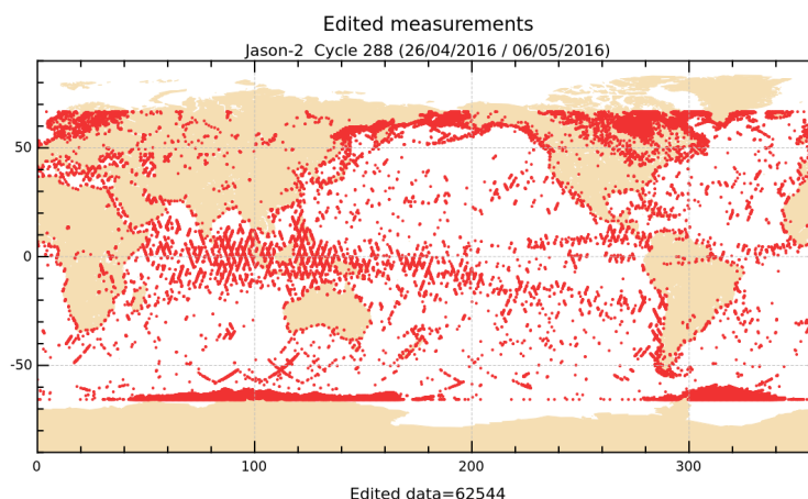
FIGURE 2 – Edited measurements for cycle 288.
