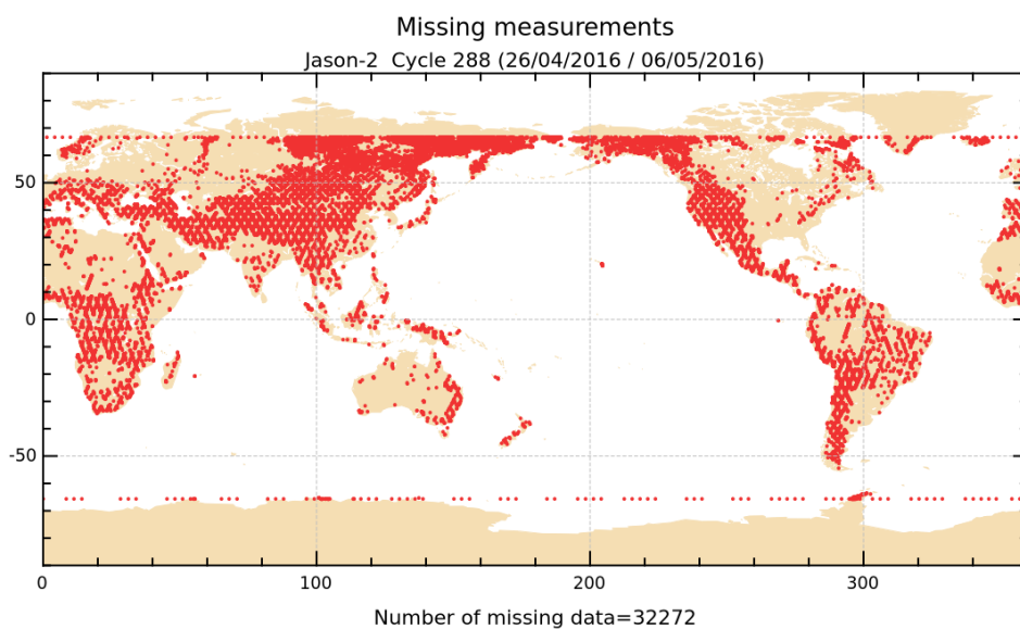
FIGURE 1 – Missing measurements for cycle 288.
