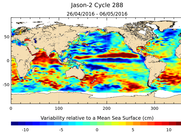
FIGURE 17 – Sea level anomaly relative to MSS for cycle 288.
