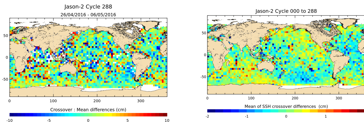
FIGURE 12 – Mean SSH at crossovers for cycle 288 (left) and over the whole Jason-2 period (right).
