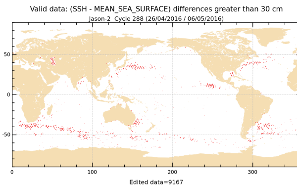
FIGURE 18 – Differences higher than a 30 cm threshold for cycle 288.
