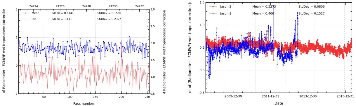
FIGURE 11 – Pass monitoring of wet troposphere differences between radiometer and ECMWF model for Jason-2 cycle 288 (left) and daily monitoring of wet troposphere differences between radiometer and ECMWF model (right).
