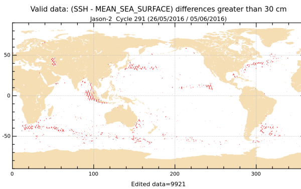
FIGURE 18 – Differences higher than a 30 cm threshold for cycle 291.
