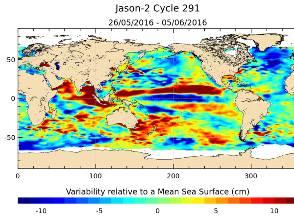
FIGURE 17 – Sea level anomaly relative to MSS for cycle 291.
