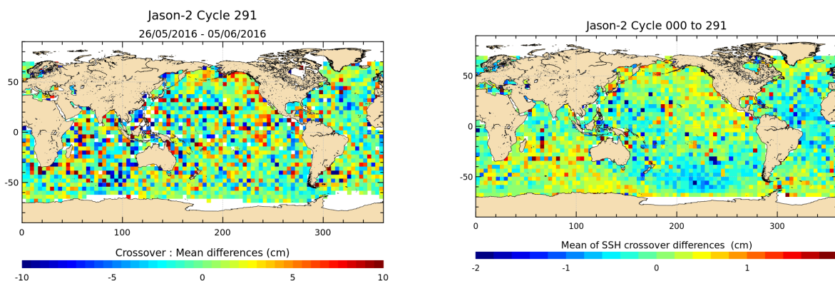
FIGURE 12 – Mean SSH at crossovers for cycle 291 (left) and over the whole Jason-2 period (right).
