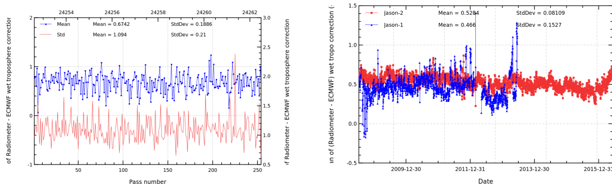
FIGURE 11 – Pass monitoring of wet troposphere differences between radiometer and ECMWF model for Jason-2 cycle 291 (left) and daily monitoring of wet troposphere differences between radiometer and ECMWF model (right).
