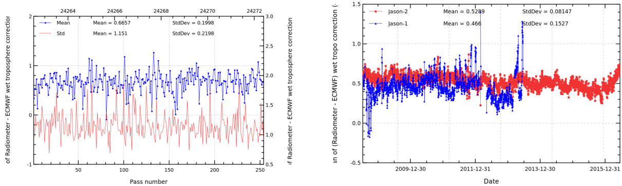
FIGURE 11 – Pass monitoring of wet troposphere differences between radiometer and ECMWF model for Jason-2 cycle 292 (left) and daily monitoring of wet troposphere differences between radiometer and ECMWF model (right).
