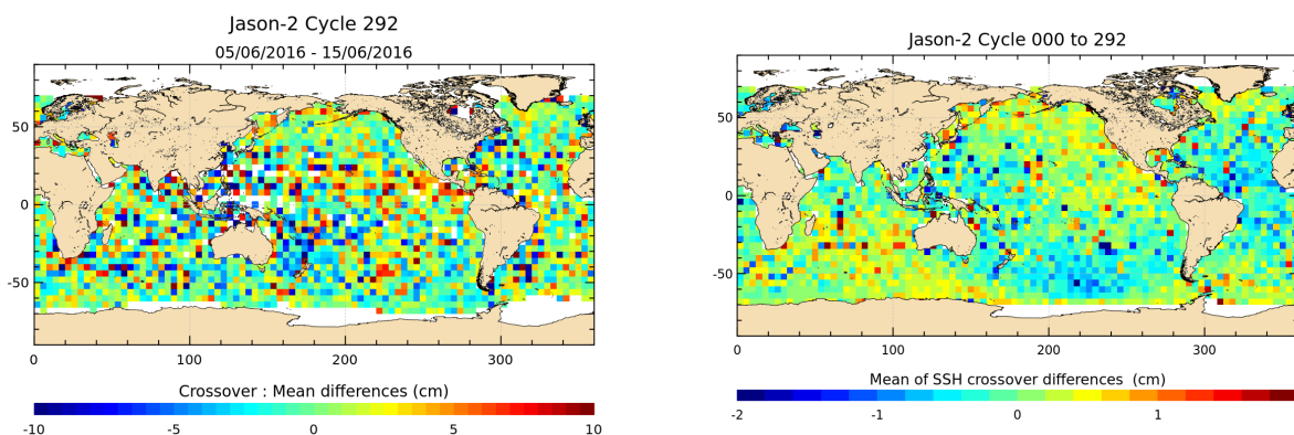
FIGURE 12 – Mean SSH at crossovers for cycle 292 (left) and over the whole Jason-2 period (right).
