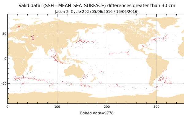
FIGURE 18 – Differences higher than a 30 cm threshold for cycle 292.
