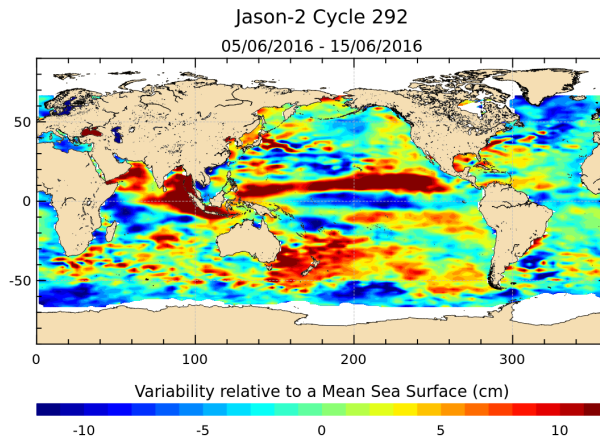
FIGURE 17 – Sea level anomaly relative to MSS for cycle 292.
