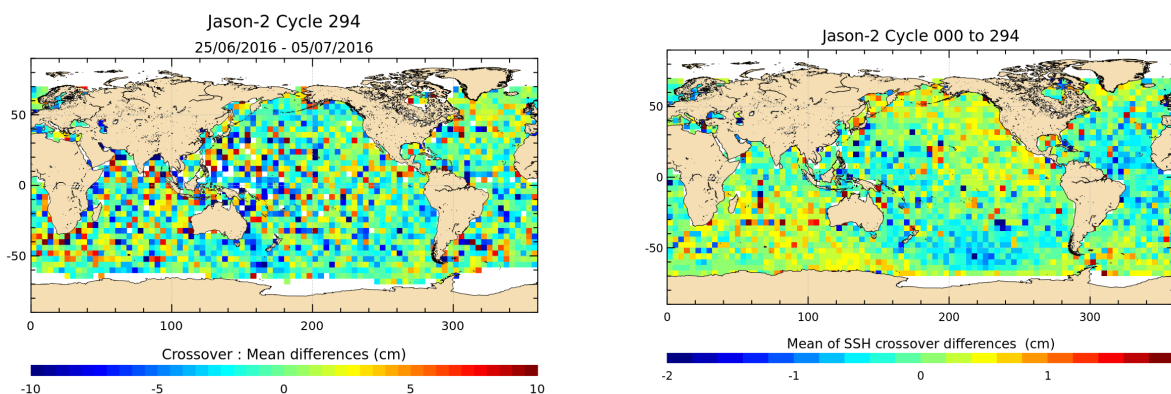
FIGURE 12 – Mean SSH at crossovers for cycle 294 (left) and over the whole Jason-2 period (right).
