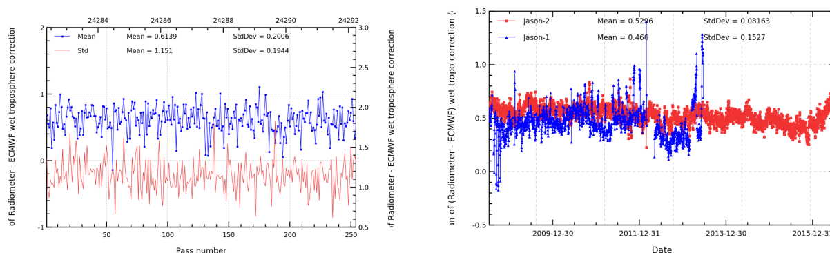
FIGURE 11 – Pass monitoring of wet troposphere differences between radiometer and ECMWF model for Jason-2 cycle 294 (left) and daily monitoring of wet troposphere differences between radiometer and ECMWF model (right).
