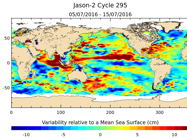
FIGURE 17 – Sea level anomaly relative to MSS for cycle 295.
