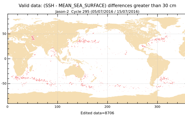
FIGURE 18 – Differences higher than a 30 cm threshold for cycle 295.
