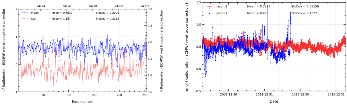
FIGURE 11 – Pass monitoring of wet troposphere differences between radiometer and ECMWF model for Jason-2 cycle 295 (left) and daily monitoring of wet troposphere differences between radiometer and ECMWF model (right).
