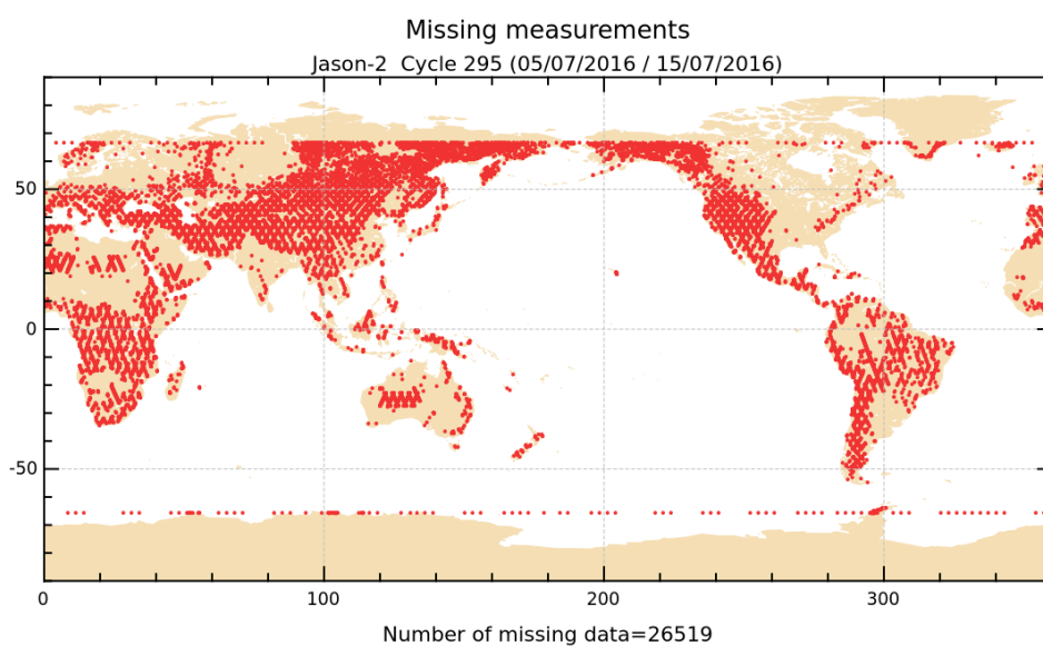
FIGURE 1 – Missing measurements for cycle 295.
