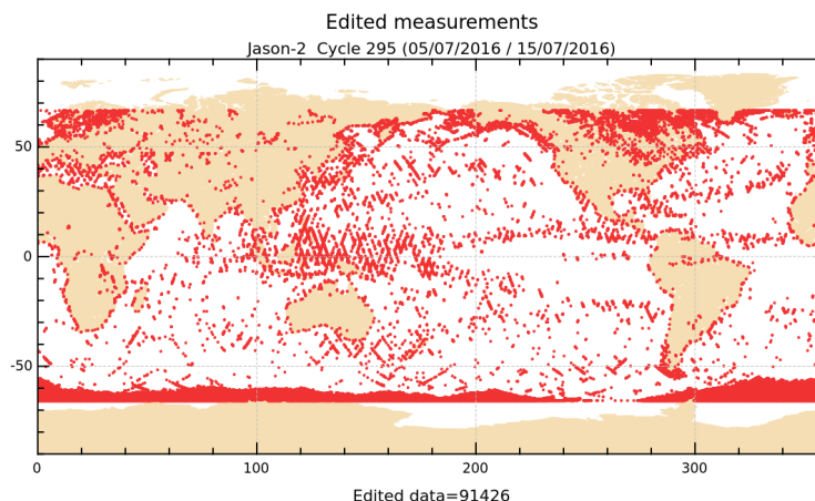
FIGURE 2 – Edited measurements for cycle 295.
