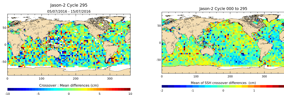
FIGURE 12 – Mean SSH at crossovers for cycle 295 (left) and over the whole Jason-2 period (right).
