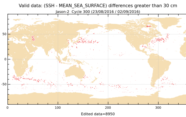
FIGURE 18 – Differences higher than a 30 cm threshold for cycle 300.
