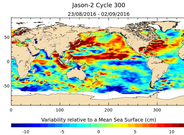
FIGURE 17 – Sea level anomaly relative to MSS for cycle 300.
