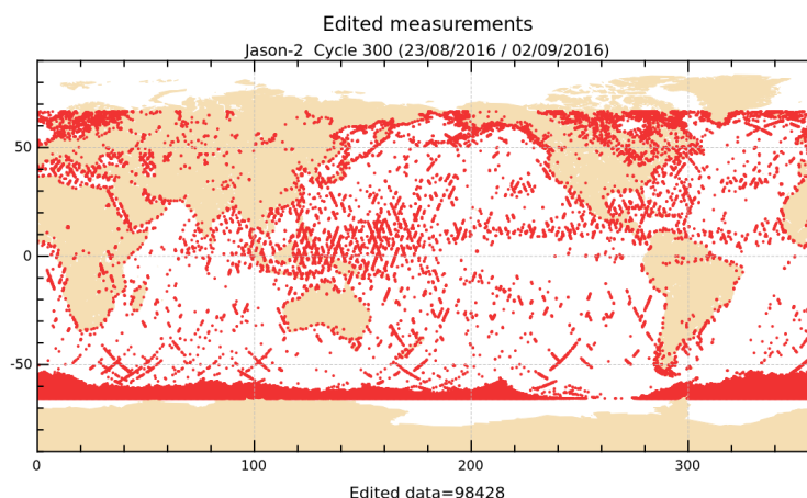
FIGURE 2 – Edited measurements for cycle 300.
