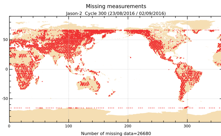
FIGURE 1 – Missing measurements for cycle 300.
