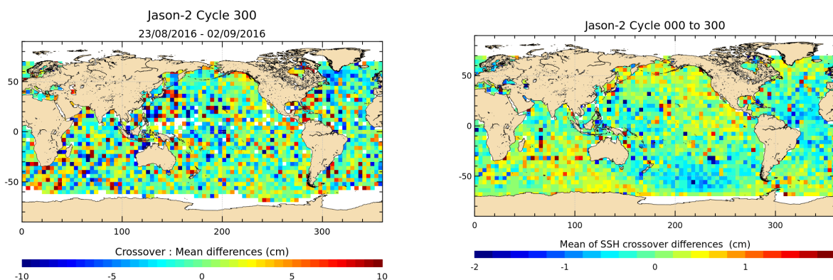
FIGURE 12 – Mean SSH at crossovers for cycle 300 (left) and over the whole Jason-2 period (right).
