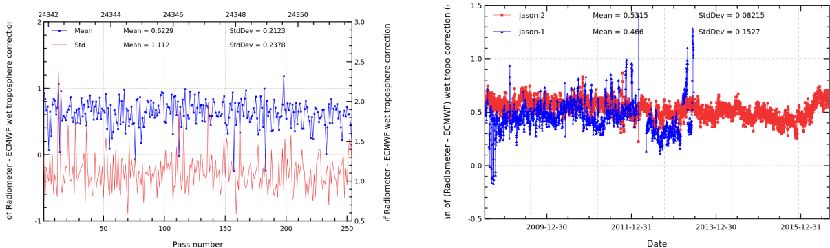
FIGURE 11 – Pass monitoring of wet troposphere differences between radiometer and ECMWF model for Jason-2 cycle 300 (left) and daily monitoring of wet troposphere differences between radiometer and ECMWF model (right).
