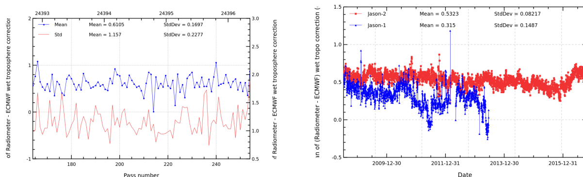
FIGURE 11 – Pass monitoring of wet troposphere differences between radiometer and ECMWF model for Jason-2 cycle 305 (left) and daily monitoring of wet troposphere differences between radiometer and ECMWF model (right).
