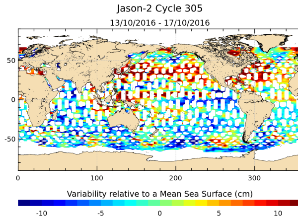
FIGURE 17 – Sea level anomaly relative to MSS for cycle 305.
