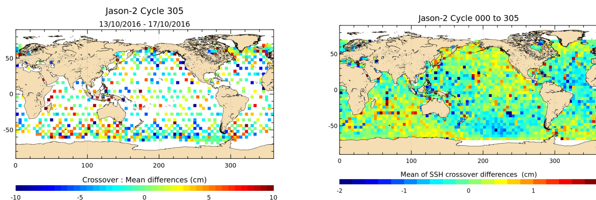
FIGURE 12 – Mean SSH at crossovers for cycle 305 (left) and over the whole Jason-2 period (right).
