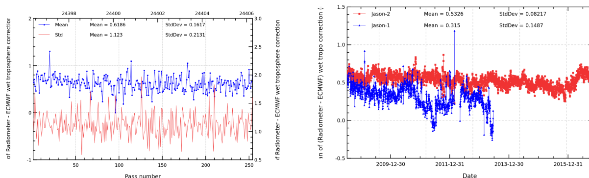
FIGURE 11 – Pass monitoring of wet troposphere differences between radiometer and ECMWF model for Jason-2 cycle 306 (left) and daily monitoring of wet troposphere differences between radiometer and ECMWF model (right).
