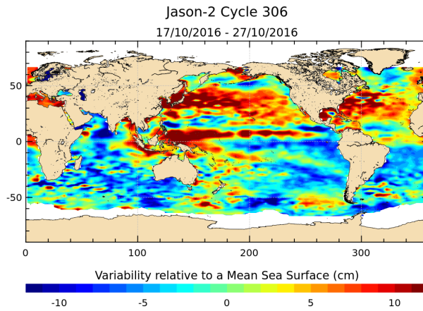
FIGURE 17 – Sea level anomaly relative to MSS for cycle 306.
