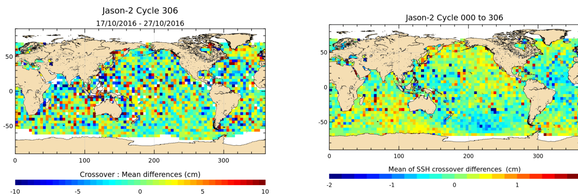
FIGURE 12 – Mean SSH at crossovers for cycle 306 (left) and over the whole Jason-2 period (right).
