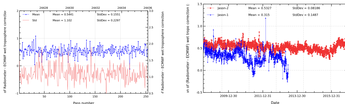
FIGURE 11 – Pass monitoring of wet troposphere differences between radiometer and ECMWF model for Jason-2 cycle 309 (left) and daily monitoring of wet troposphere differences between radiometer and ECMWF model (right).
