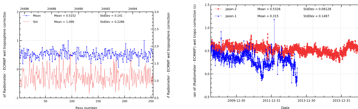
FIGURE 11 – Pass monitoring of wet troposphere differences between radiometer and ECMWF model for Jason-2 cycle 315 (left) and daily monitoring of wet troposphere differences between radiometer and ECMWF model (right).
