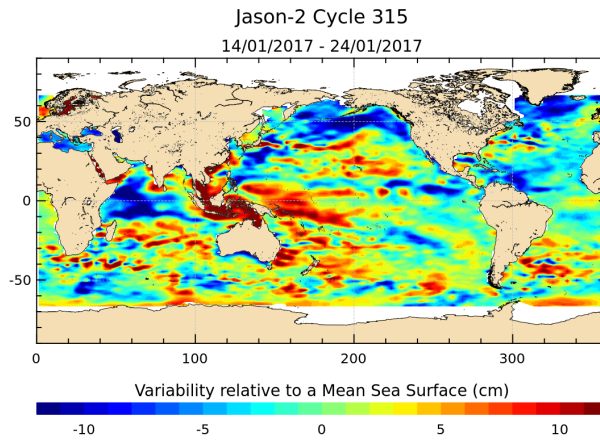
FIGURE 17 – Sea level anomaly relative to MSS for cycle 315.
