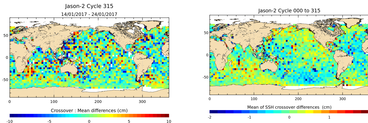
FIGURE 12 – Mean SSH at crossovers for cycle 315 (left) and over the whole Jason-2 period (right).
