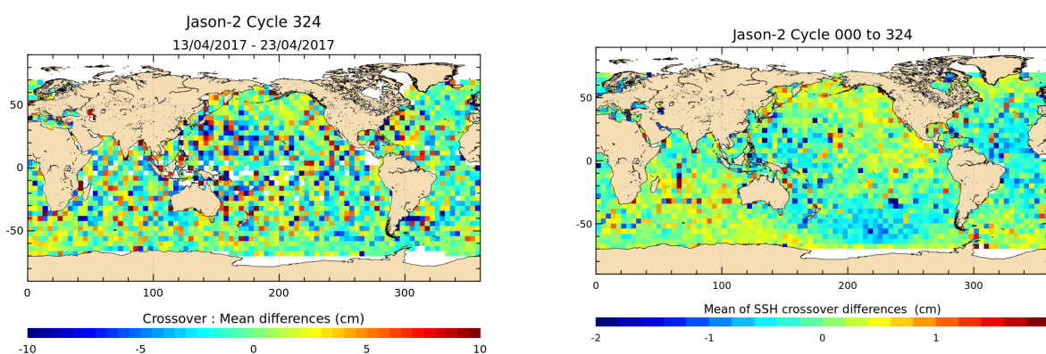
FIGURE 12 – Mean SSH at crossovers for cycle 324 (left) and over the whole Jason-2 period (right).
