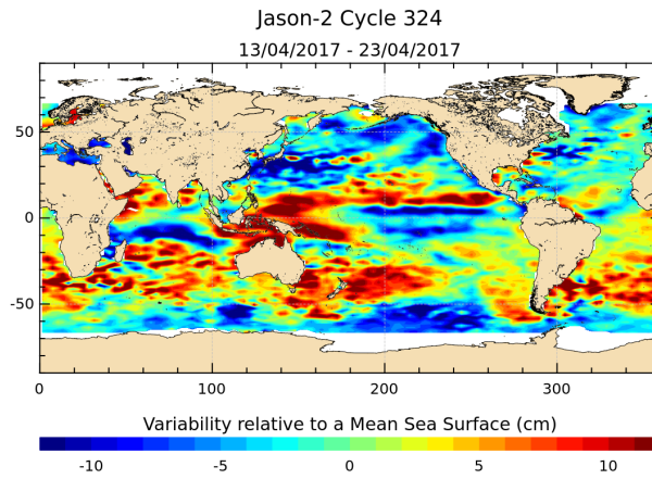
FIGURE 17 – Sea level anomaly relative to MSS for cycle 324.
