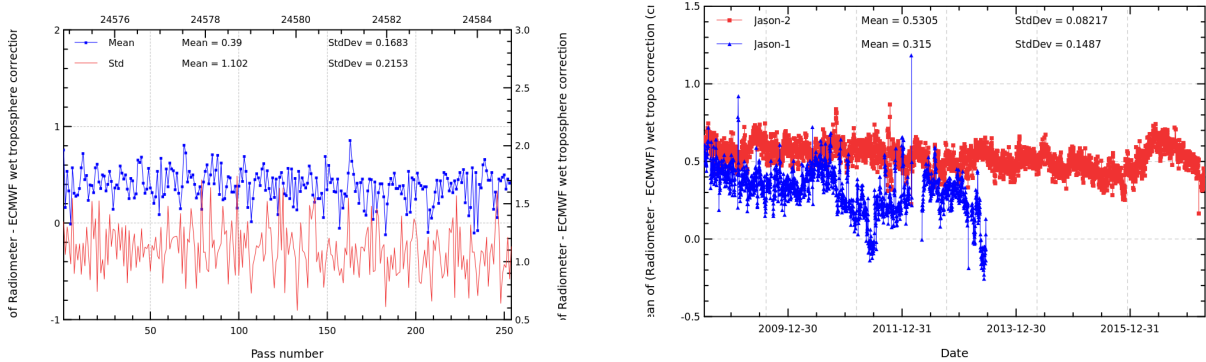
FIGURE 11 – Pass monitoring of wet troposphere differences between radiometer and ECMWF model for Jason-2 cycle 324 (left) and daily monitoring of wet troposphere differences between radiometer and ECMWF model (right).
