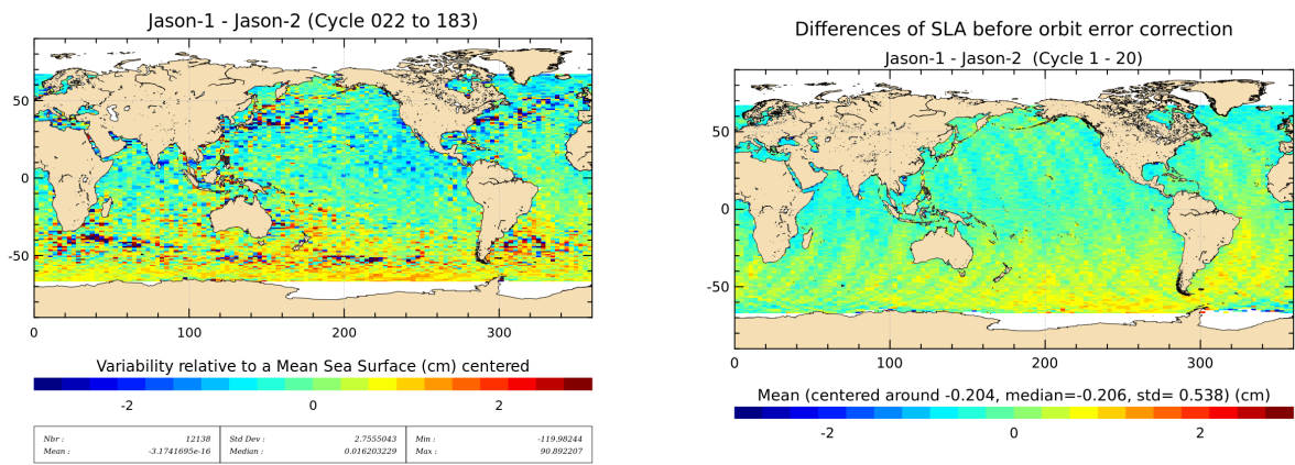
FIGURE 19 – Jason-1 – Jason-2 SLA differences averaged over Jason-2 period from cycle 022 until cycle 183 (left), and for tandem phase (cycle 001 to 020) (right).
