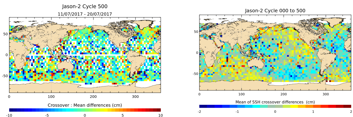
FIGURE 12 – Mean SSH at crossovers for cycle 500 (left) and over the whole Jason-2 period (right).
