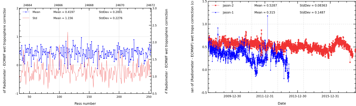
FIGURE 11 – Pass monitoring of wet troposphere differences between radiometer and ECMWF model for Jason-2 cycle 500 (left) and daily monitoring of wet troposphere differences between radiometer and ECMWF model (right).
