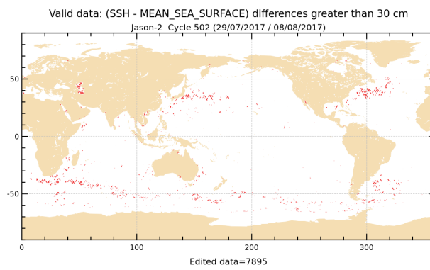
FIGURE 17 – Sea level anomaly relative to MSS for cycle 502.
