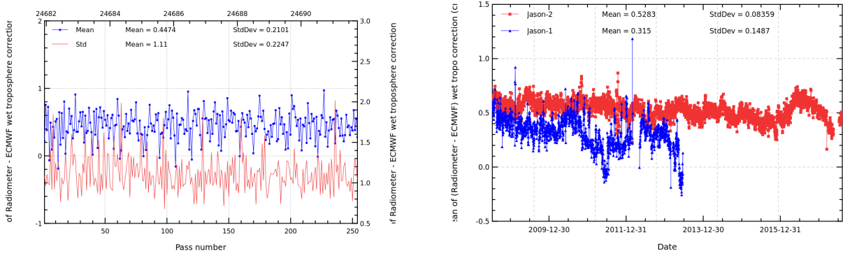
FIGURE 11 – Pass monitoring of wet troposphere differences between radiometer and ECMWF model for Jason-2 cycle 502 (left) and daily monitoring of wet troposphere differences between radiometer and ECMWF model (right).
