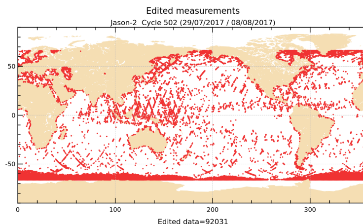
FIGURE 2 – Edited measurements for cycle 502.
