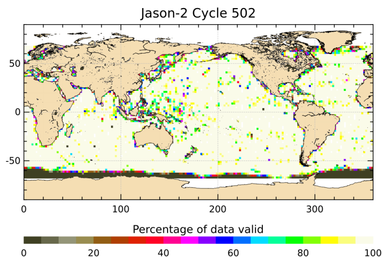
FIGURE 3 – Percentage of valid measurements for cycle 502.
