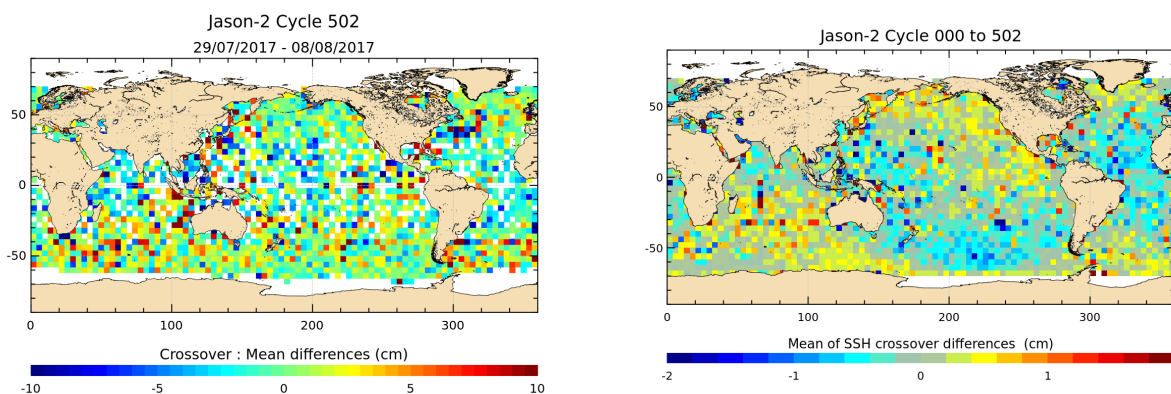
FIGURE 12 – Mean SSH at crossovers for cycle 502 (left) and over the whole Jason-2 period (right).
