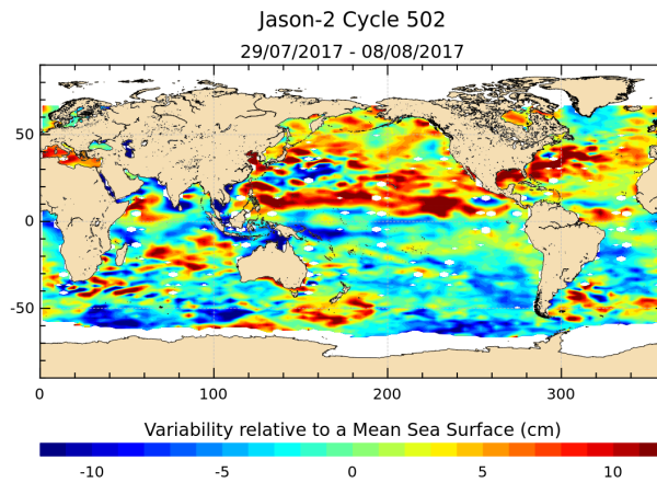
FIGURE 17 – Sea level anomaly relative to MSS for cycle 502.
