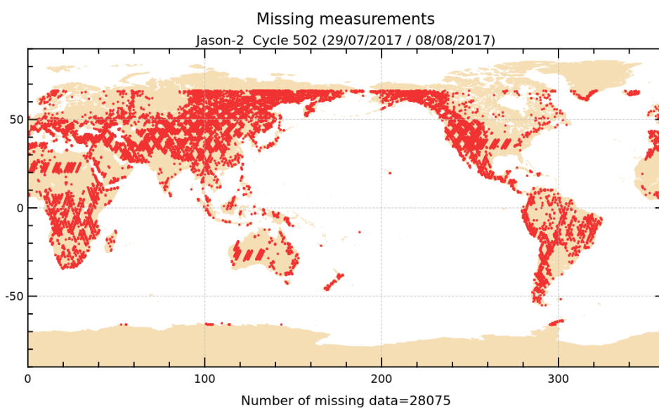
FIGURE 1 – Missing measurements for cycle 502.
