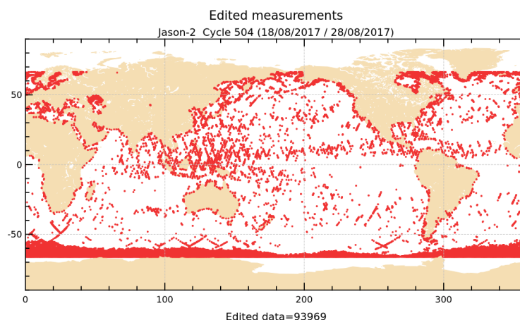
FIGURE 2 – Edited measurements for cycle 504.
