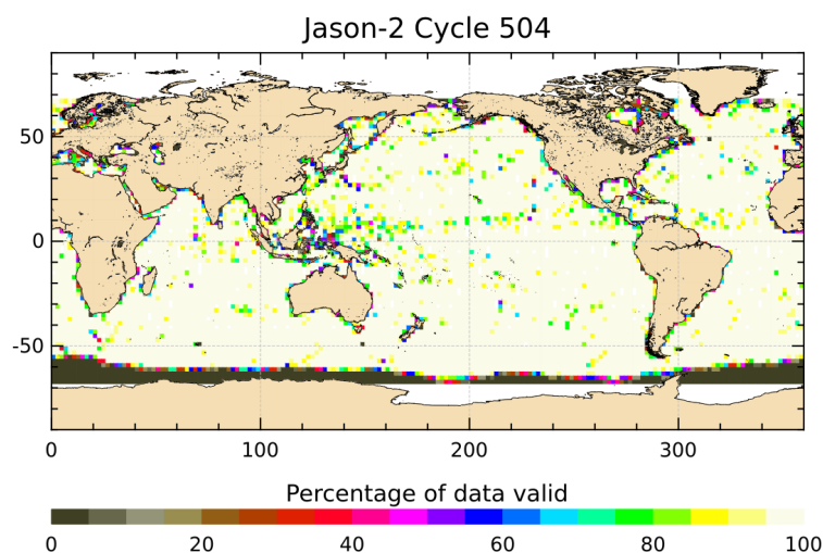
FIGURE 3 – Percentage of valid measurements for cycle 504.
