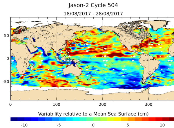
FIGURE 18 – Sea level anomaly relative to MSS for cycle 504.
