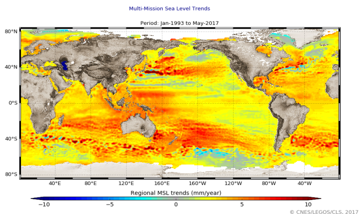
FIGURE 23 – Regional MSL trends from 1993 onwards.
