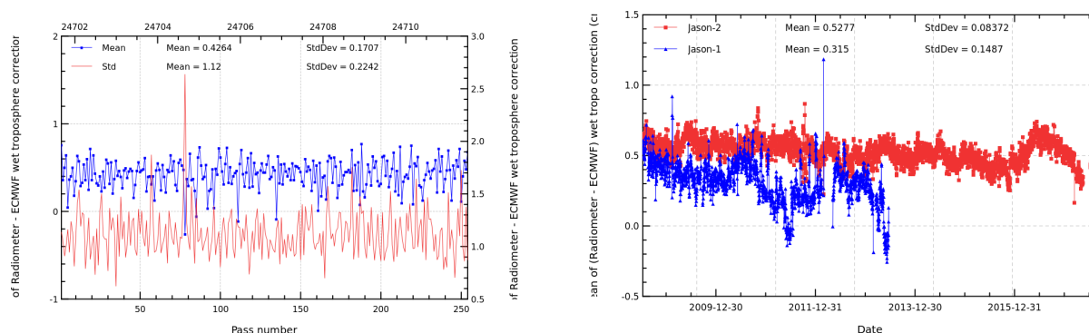
FIGURE 12 – Pass monitoring of wet troposphere differences between radiometer and ECMWF model for Jason-2 cycle 504 (left) and daily monitoring of wet troposphere differences between radiometer and ECMWF model (right).
