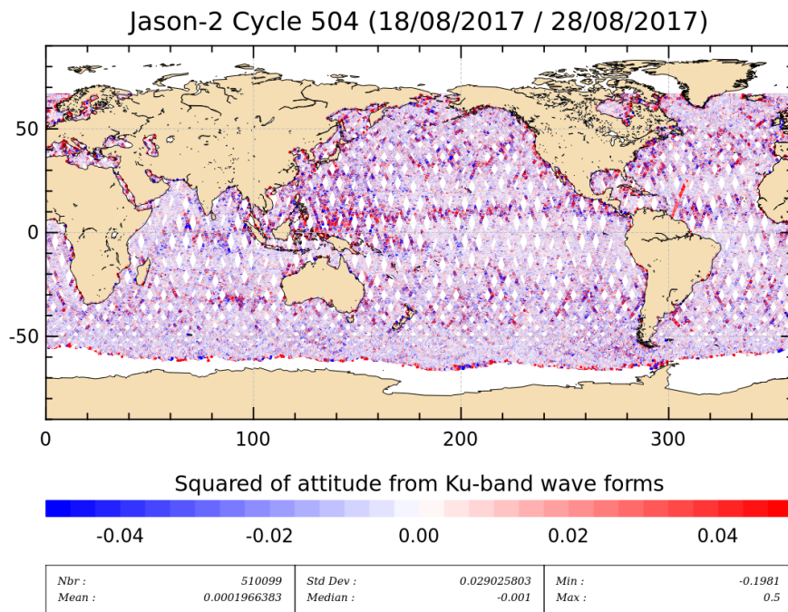
FIGURE 4 – Apparent squared mispointing from waveforms for cycle 504.
