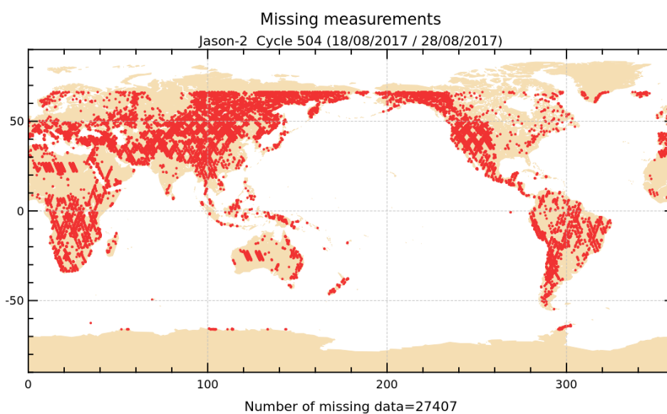
FIGURE 1 – Missing measurements for cycle 504.
