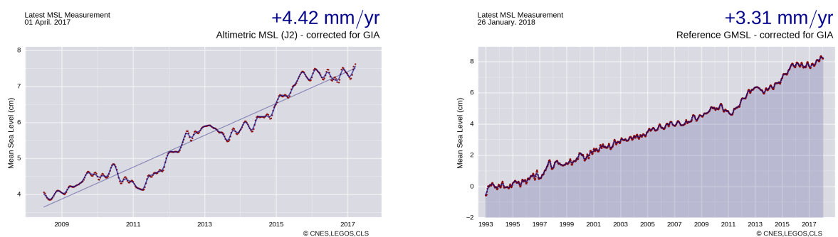
FIGURE 22 – Global MSL on Jason-2 mission (left) and with reference missions from 1993 onwards (right).
