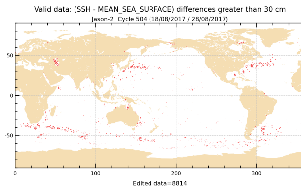
FIGURE 18 – Sea level anomaly relative to MSS for cycle 504.
