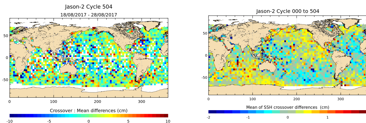
FIGURE 13 – Mean SSH at crossovers for cycle 504 (left) and over the whole Jason-2 period (right).
