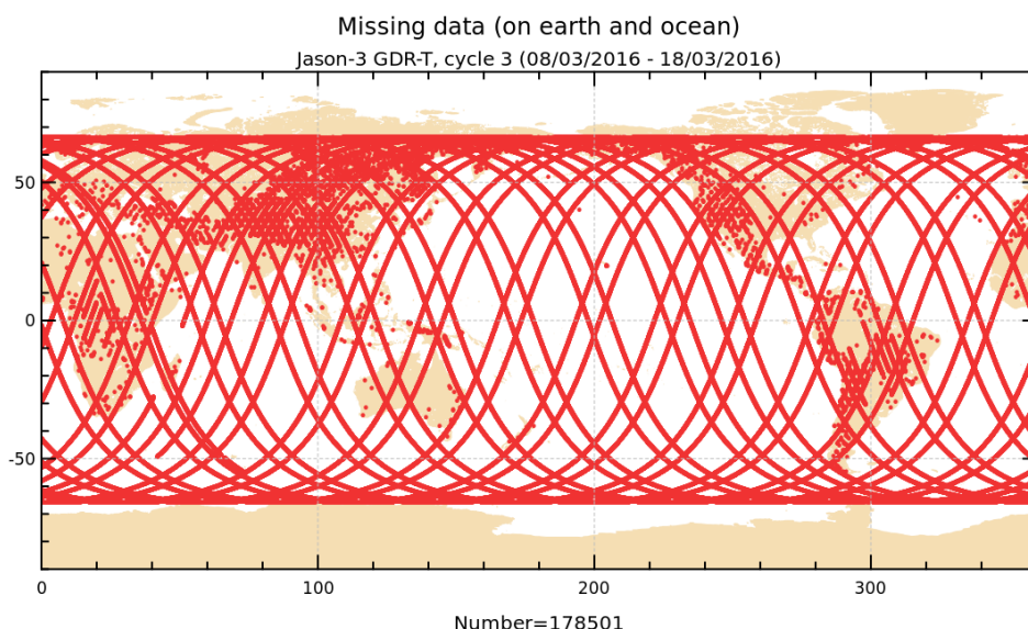
FIGURE 1 – Missing measurements for cycle 003.
