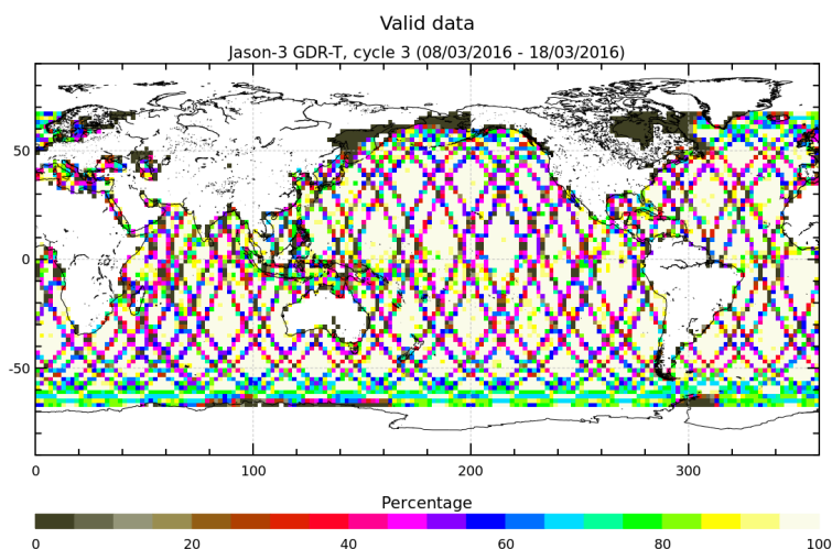
FIGURE 3 – Percentage of valid measurements for cycle 003.
