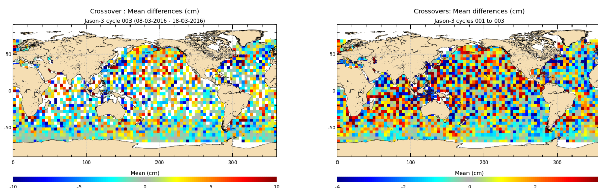
FIGURE 13 – Mean SSH at crossovers for cycle 003 (left) and over the whole Jason-3 period (right).
