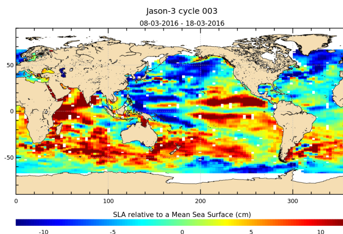
FIGURE 18 – Sea level anomaly relative to MSS for cycle 003.
