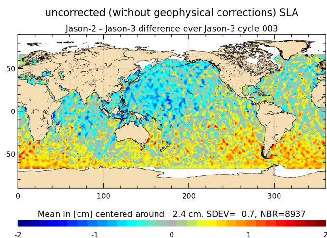
FIGURE 19 – Jason-2 – Jason-3 SLA differences (without corrections) for cycle 003.
