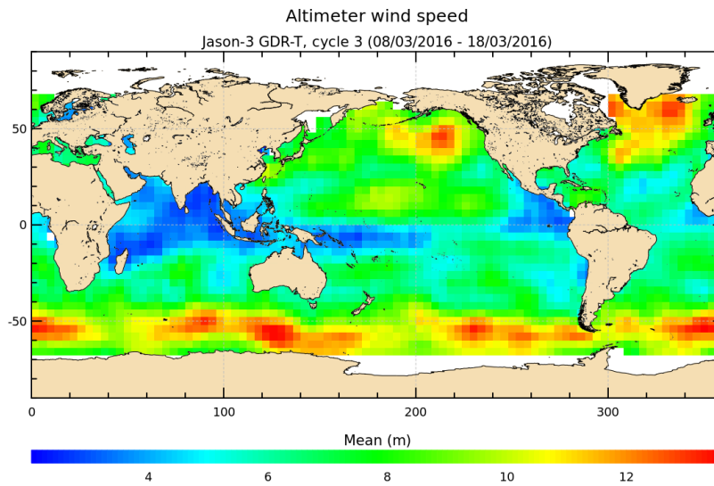
FIGURE 10 – Altimeter wind speed for cycle 003.
