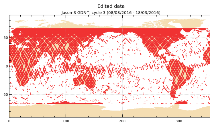
FIGURE 2 – Edited measurements for cycle 003.
