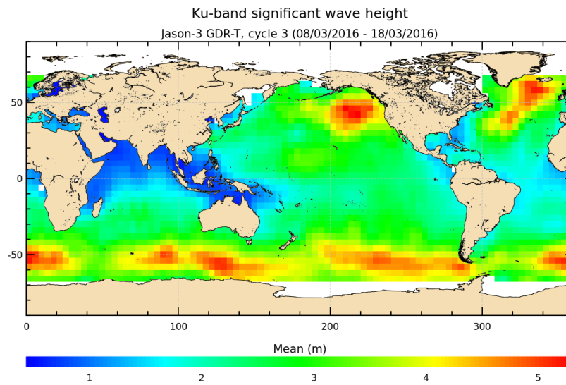
FIGURE 6 – Significant wave height for cycle 003.
