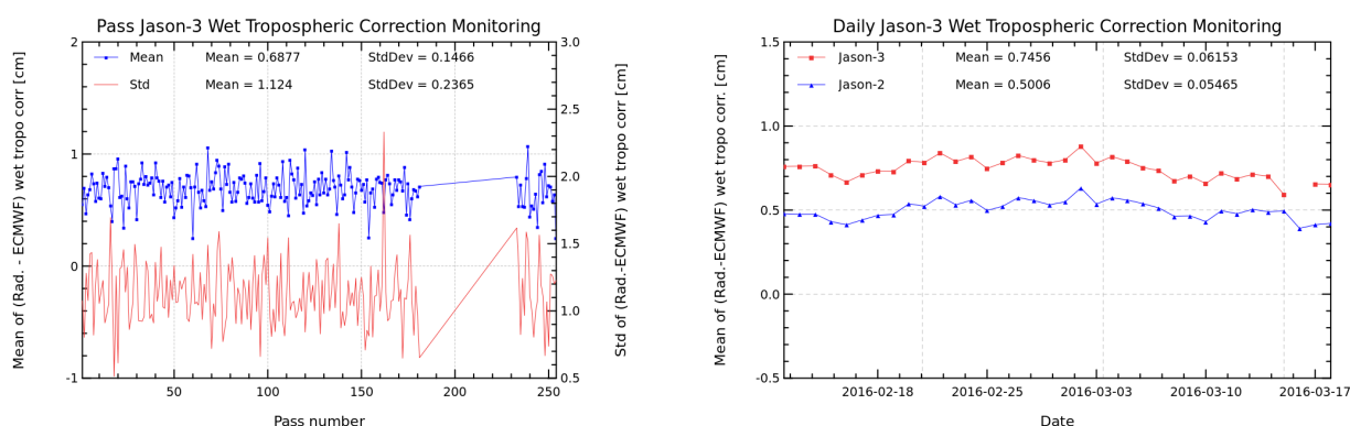
FIGURE 12 – Pass monitoring of wet troposphere differences between radiometer and ECMWF model for Jason-3 cycle 003 (left) and Jason-3 versus Jason-2 daily monitoring of wet troposphere differences between radiometer and ECMWF model (right).
