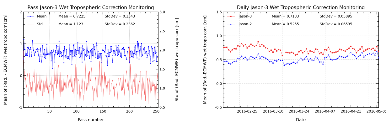
FIGURE 11 – Pass monitoring of wet troposphere differences between radiometer and ECMWF model for Jason-3 cycle 008 (left) and Jason-3 versus Jason-2 daily monitoring of wet troposphere differences between radiometer and ECMWF model (right).
