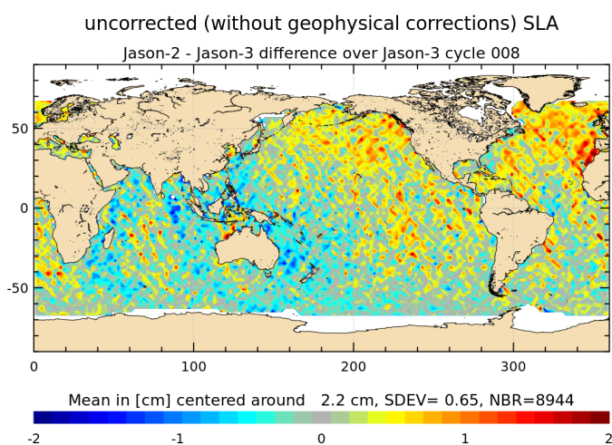
FIGURE 18 – Jason-2 – Jason-3 SLA differences (without corrections) for cycle 008.
