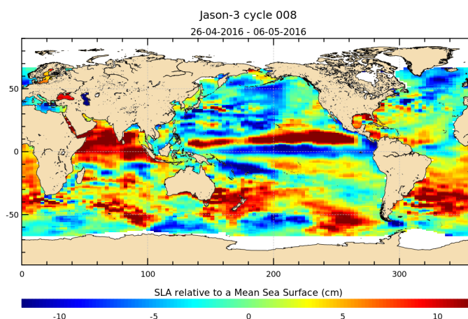
FIGURE 17 – Sea level anomaly relative to MSS for cycle 008.
