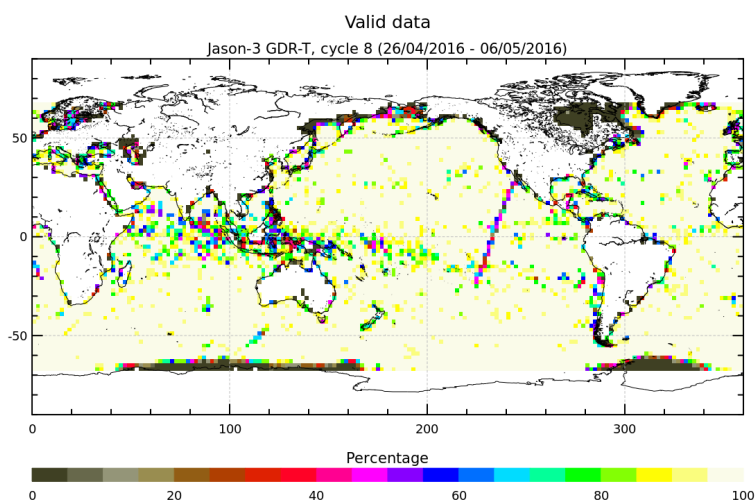
FIGURE 3 – Percentage of valid measurements for cycle 008.
