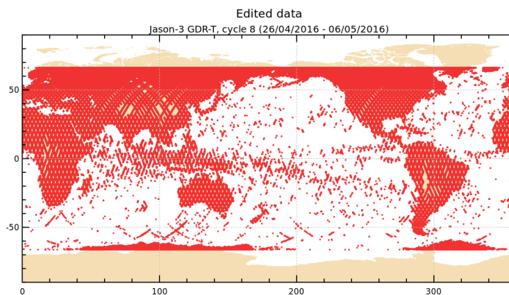
FIGURE 2 – Edited measurements for cycle 008.
