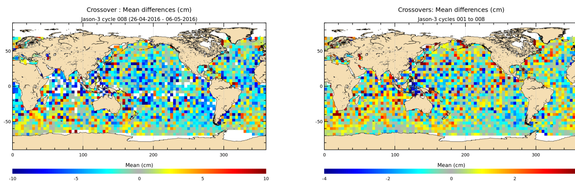
FIGURE 12 – Mean SSH at crossovers for cycle 008 (left) and over the whole Jason-3 period (right).
