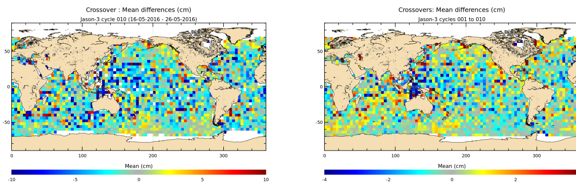
FIGURE 12 – Mean SSH at crossovers for cycle 010 (left) and over the whole Jason-3 period (right).
