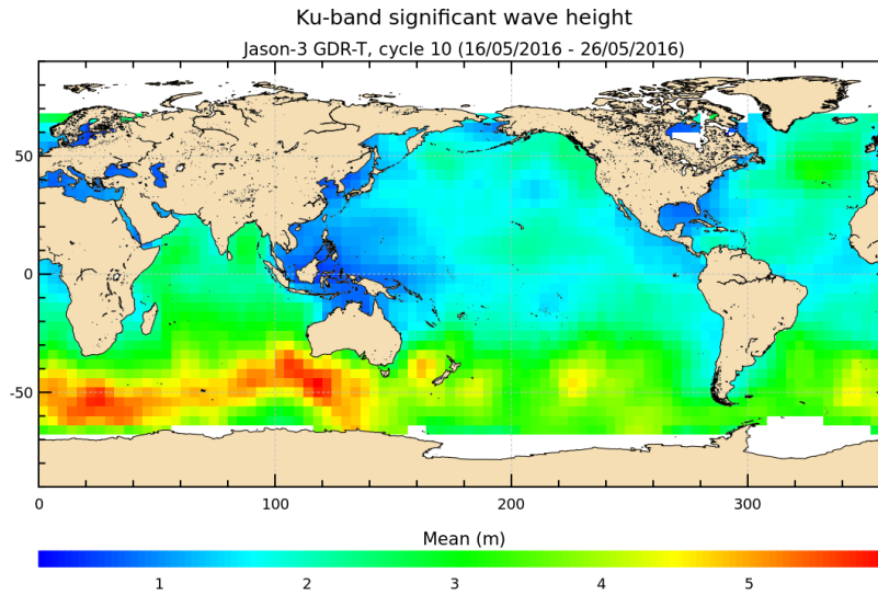
FIGURE 5 – Significant wave height for cycle 010.
