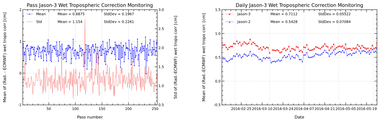
FIGURE 11 – Pass monitoring of wet troposphere differences between radiometer and ECMWF model for Jason-3 cycle 010 (left) and Jason-3 versus Jason-2 daily monitoring of wet troposphere differences between radiometer and ECMWF model (right).
