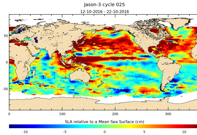
FIGURE 17 – Sea level anomaly relative to MSS for cycle 025.
