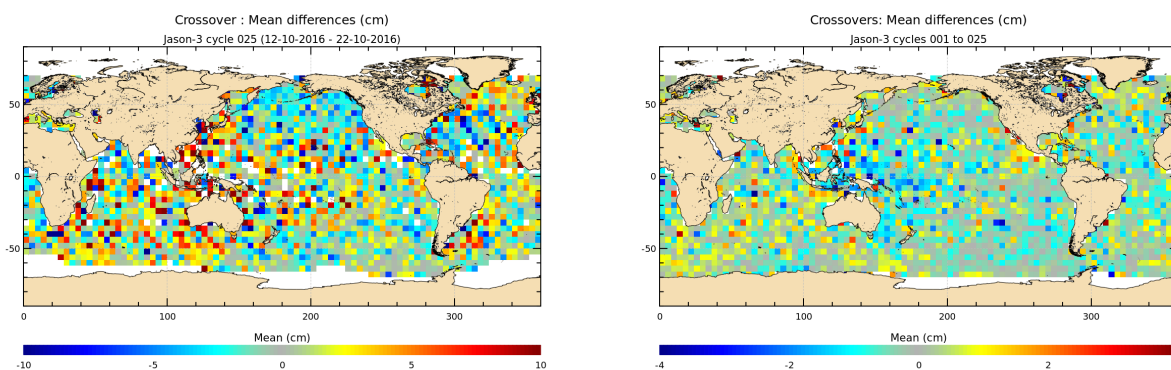
FIGURE 12 – Mean SSH at crossovers for cycle 025 (left) and over the whole Jason-3 period (right).
