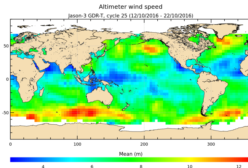
FIGURE 9 – Altimeter wind speed for cycle 025.
