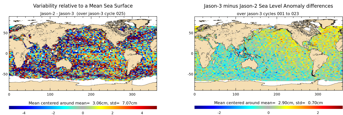
FIGURE 18 – Jason-2 – Jason-3 SLA differences averaged over Jason-3 period for cycle 025 (left), and for tandem phase (cycle 001 to 023) (right).
