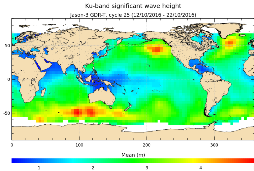
FIGURE 5 – Significant wave height for cycle 025.
