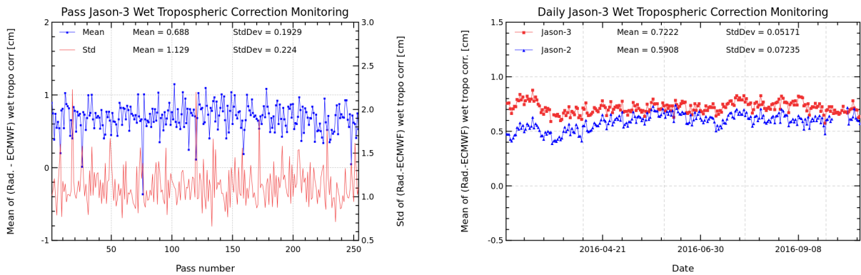
FIGURE 11 – Pass monitoring of wet troposphere differences between radiometer and ECMWF model for Jason-3 cycle 025 (left) and Jason-3 versus Jason-2 daily monitoring of wet troposphere differences between radiometer and ECMWF model (right).
