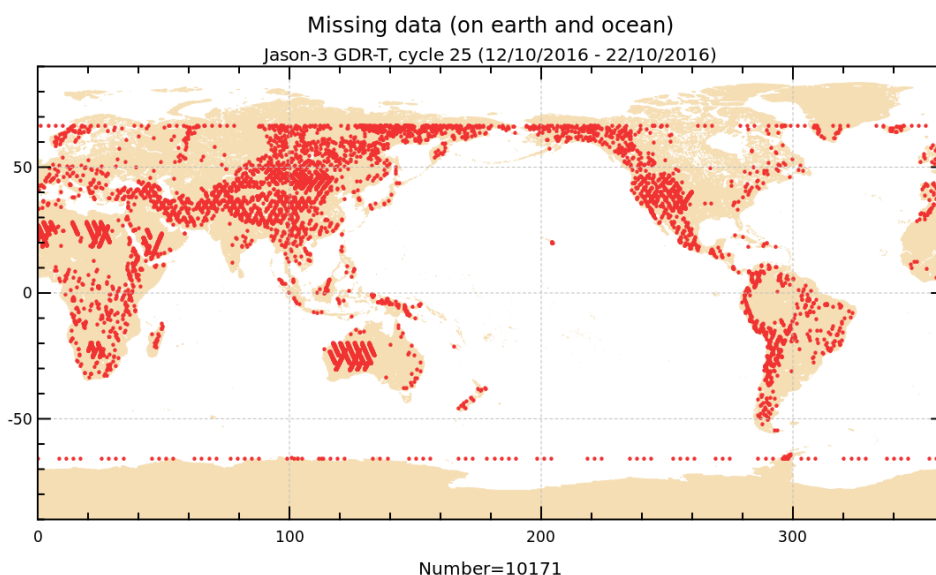
FIGURE 1 – Missing measurements for cycle 025.
