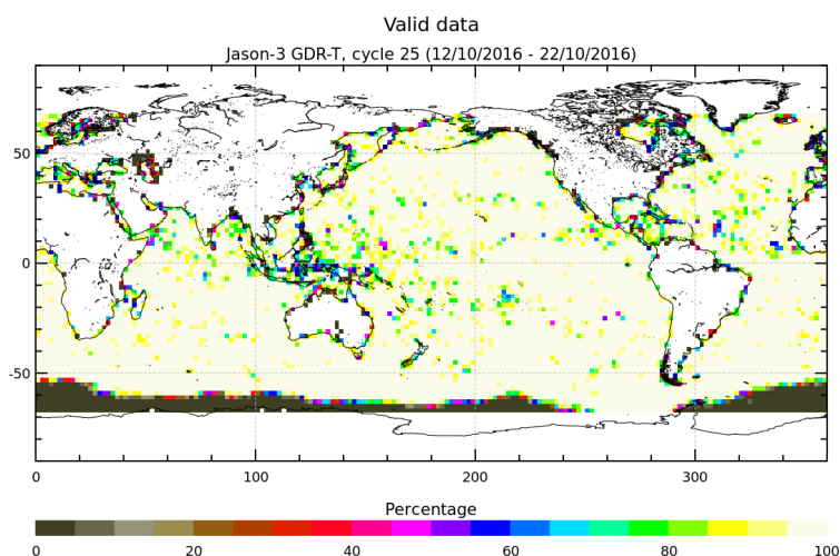
FIGURE 3 – Percentage of valid measurements for cycle 025.
