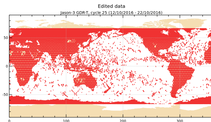
FIGURE 2 – Edited measurements for cycle 025.
