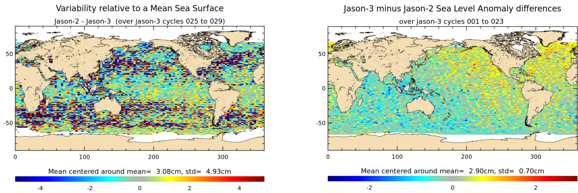
FIGURE 18 – Jason-2 – Jason-3 SLA differences averaged over Jason-3 period from cycle 025 until cycle 029 (left), and for tandem phase (cycle 001 to 023) (right).
