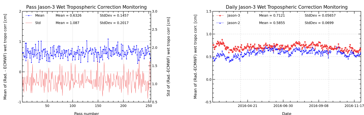
FIGURE 11 – Pass monitoring of wet troposphere differences between radiometer and ECMWF model for Jason-3 cycle 029 (left) and Jason-3 versus Jason-2 daily monitoring of wet troposphere differences between radiometer and ECMWF model (right).
