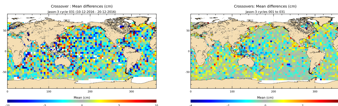
FIGURE 12 – Mean SSH at crossovers for cycle 031 (left) and over the whole Jason-3 period (right).
