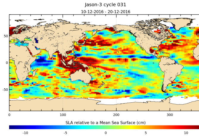
FIGURE 17 – Sea level anomaly relative to MSS for cycle 031.
