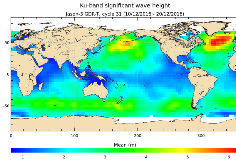
FIGURE 5 – Significant wave height for cycle 031.
