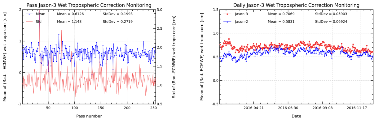
FIGURE 11 – Pass monitoring of wet troposphere differences between radiometer and ECMWF model for Jason-3 cycle 031 (left) and Jason-3 versus Jason-2 daily monitoring of wet troposphere differences between radiometer and ECMWF model (right).
