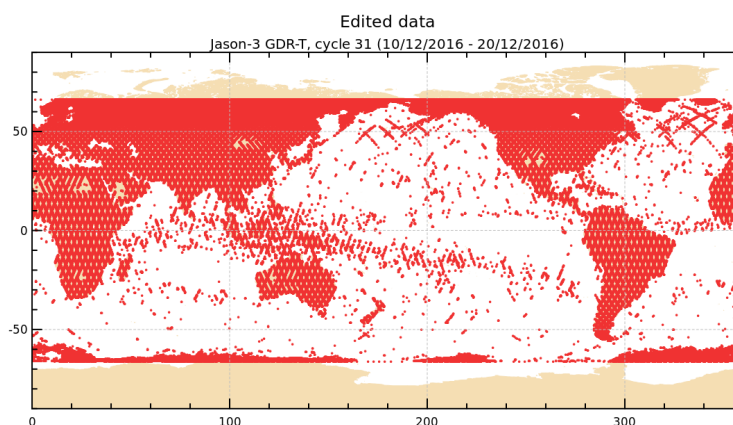
FIGURE 2 – Edited measurements for cycle 031.
