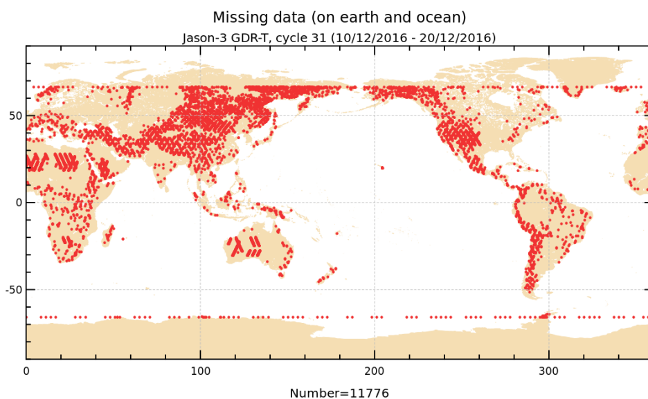
FIGURE 1 – Missing measurements for cycle 031.
