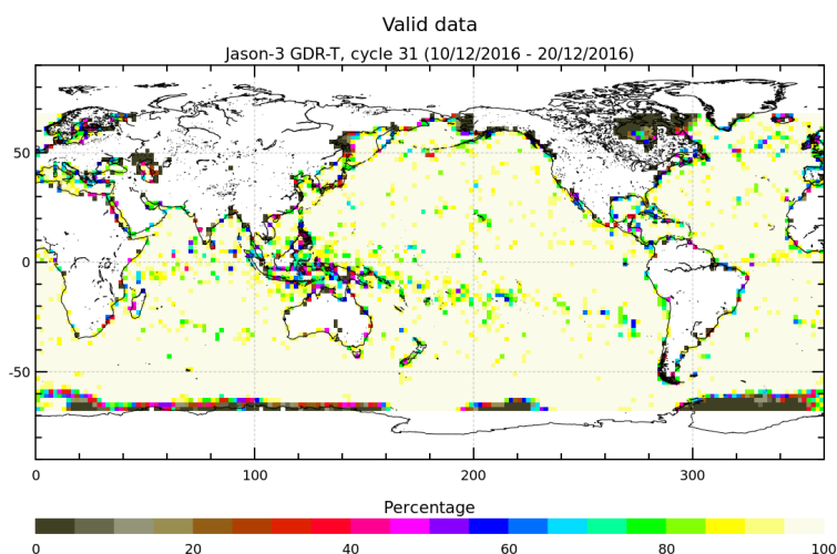
FIGURE 3 – Percentage of valid measurements for cycle 031.
