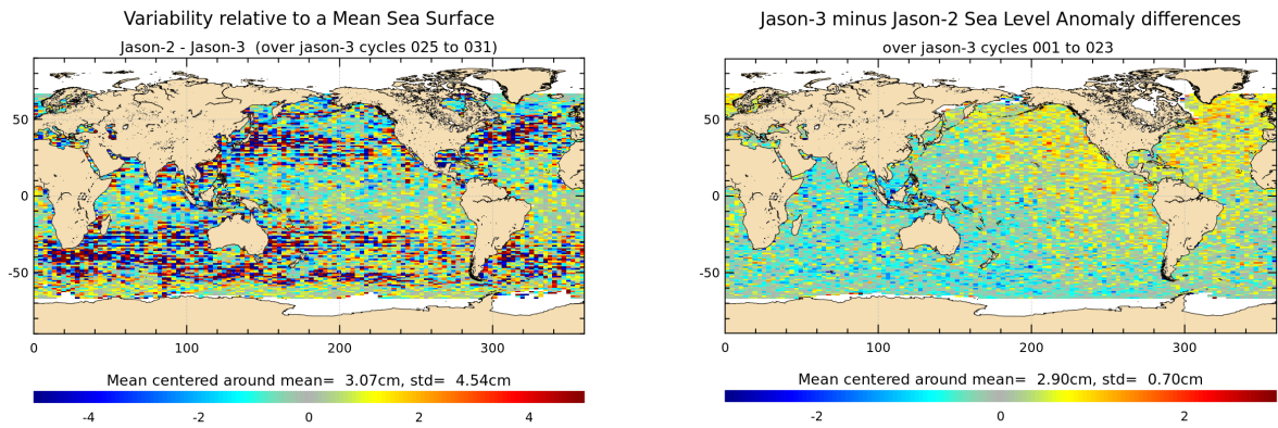
FIGURE 18 – Jason-2 – Jason-3 SLA differences averaged over Jason-3 period from cycle 025 until cycle 031 (left), and for tandem phase (cycle 001 to 023) (right).
