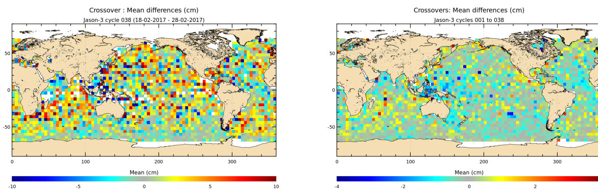
FIGURE 12 – Mean SSH at crossovers for cycle 038 (left) and over the whole Jason-3 period (right).
