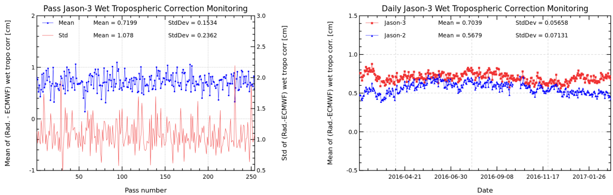
FIGURE 11 – Pass monitoring of wet troposphere differences between radiometer and ECMWF model for Jason-3 cycle 038 (left) and Jason-3 versus Jason-2 daily monitoring of wet troposphere differences between radiometer and ECMWF model (right).
