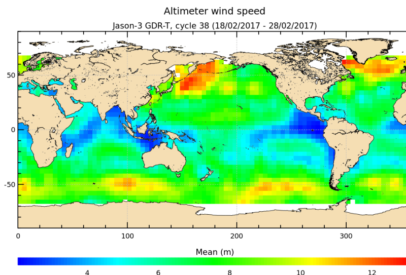
FIGURE 9 – Altimeter wind speed for cycle 038.
