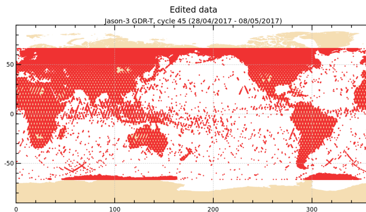
FIGURE 2 – Edited measurements for cycle 045.
