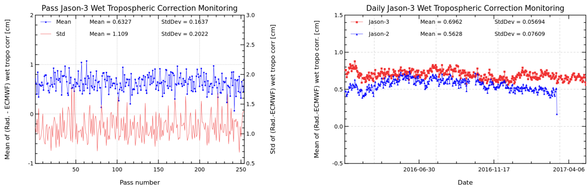
FIGURE 11 – Pass monitoring of wet troposphere differences between radiometer and ECMWF model for Jason-3 cycle 045 (left) and Jason-3 versus Jason-2 daily monitoring of wet troposphere differences between radiometer and ECMWF model (right).
