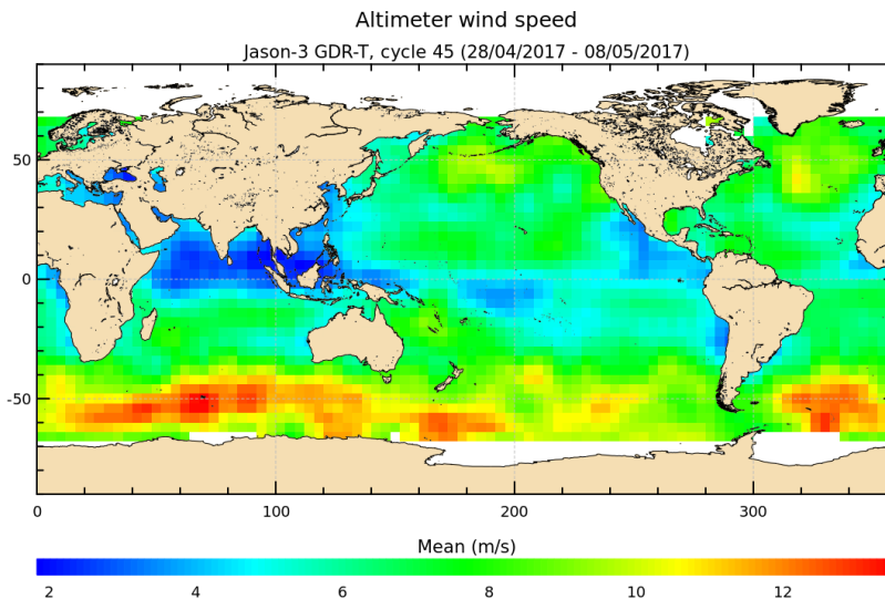
FIGURE 9 – Altimeter wind speed for cycle 045.
