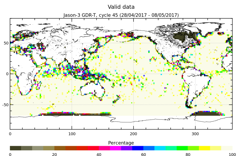
FIGURE 3 – Percentage of valid measurements for cycle 045.
