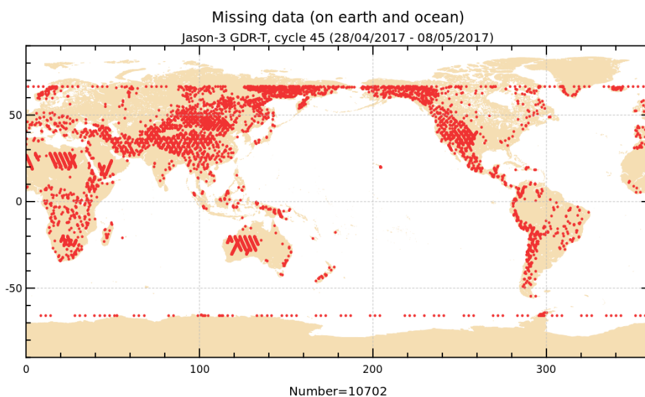
FIGURE 1 – Missing measurements for cycle 045.
