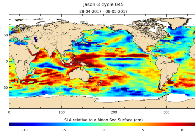
FIGURE 17 – Sea level anomaly relative to MSS for cycle 045.
