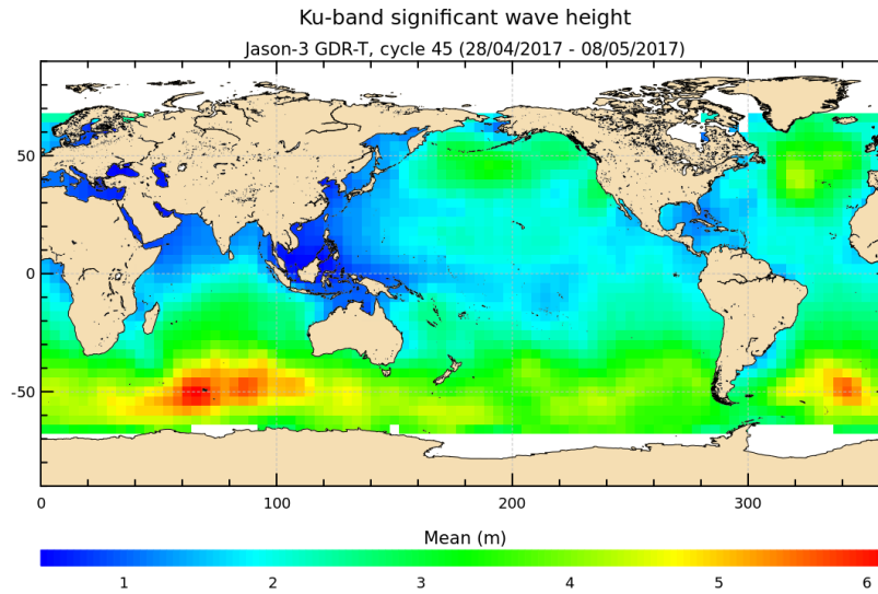
FIGURE 5 – Significant wave height for cycle 045.
