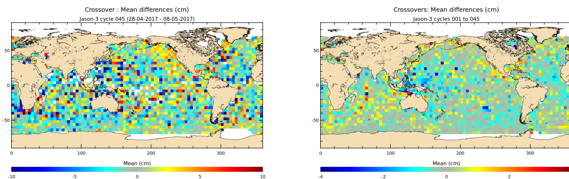
FIGURE 12 – Mean SSH at crossovers for cycle 045 (left) and over the whole Jason-3 period (right).
