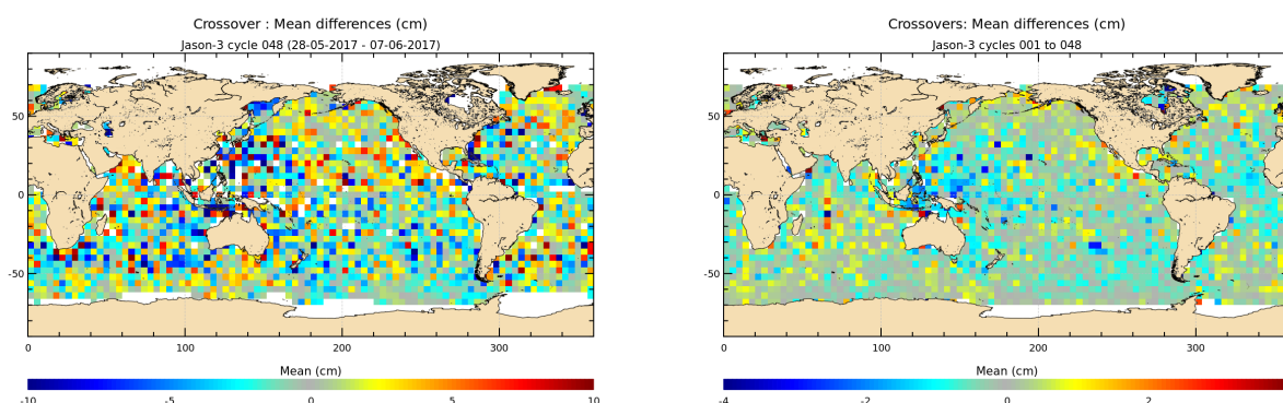
FIGURE 12 – Mean SSH at crossovers for cycle 048 (left) and over the whole Jason-3 period (right).
