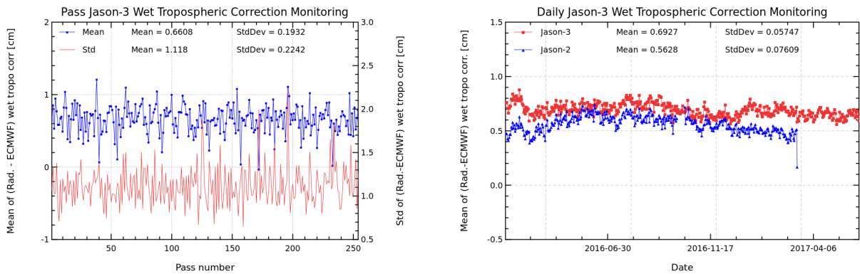
FIGURE 11 – Pass monitoring of wet troposphere differences between radiometer and ECMWF model for Jason-3 cycle 048 (left) and Jason-3 versus Jason-2 daily monitoring of wet troposphere differences between radiometer and ECMWF model (right).
