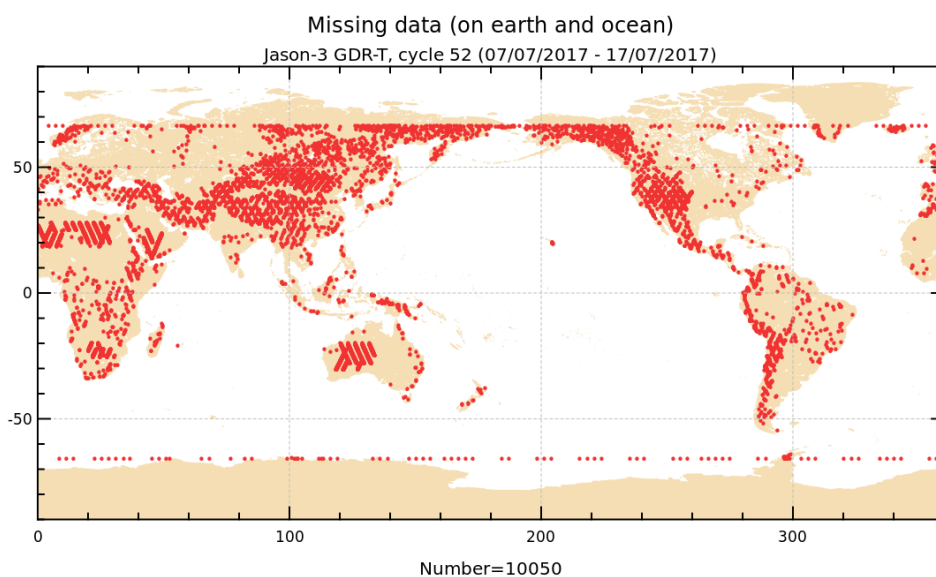
FIGURE 1 – Missing measurements for cycle 052.
