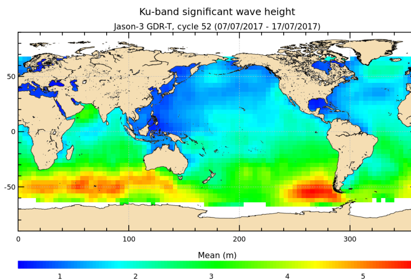
FIGURE 5 – Significant wave height for cycle 052.
