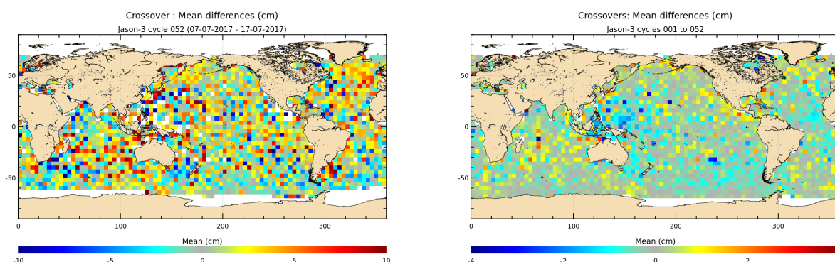
FIGURE 12 – Mean SSH at crossovers for cycle 052 (left) and over the whole Jason-3 period (right).
