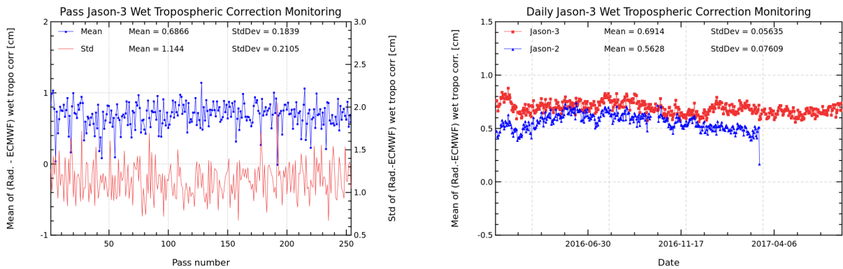
FIGURE 11 – Pass monitoring of wet troposphere differences between radiometer and ECMWF model for Jason-3 cycle 052 (left) and Jason-3 versus Jason-2 daily monitoring of wet troposphere differences between radiometer and ECMWF model (right).
