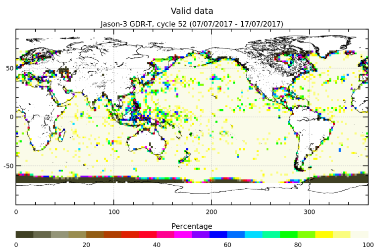
FIGURE 3 – Percentage of valid measurements for cycle 052.
