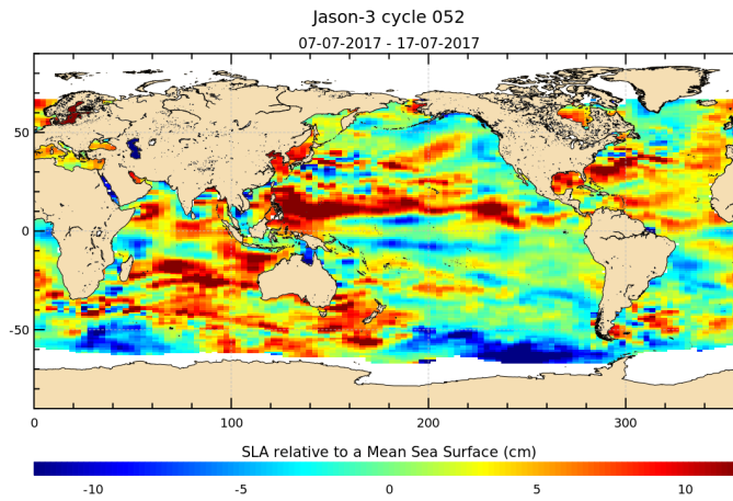
FIGURE 17 – Sea level anomaly relative to MSS for cycle 052.
