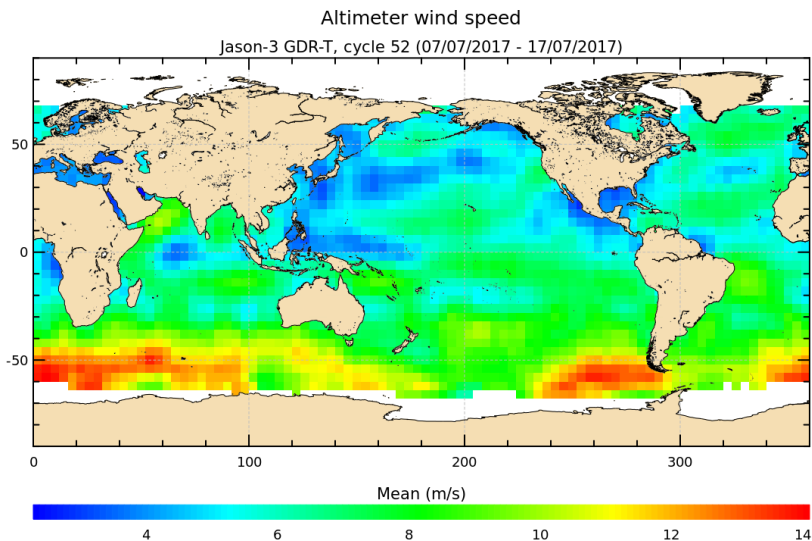
FIGURE 9 – Altimeter wind speed for cycle 052.
