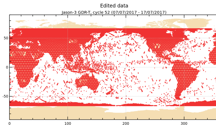
FIGURE 2 – Edited measurements for cycle 052.
