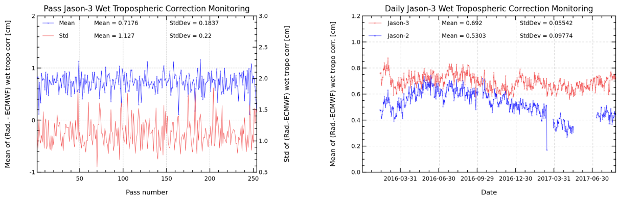
FIGURE 11 – Pass monitoring of wet troposphere differences between radiometer and ECMWF model for Jason-3 cycle 056 (left) and Jason-3 versus Jason-2 daily monitoring of wet troposphere differences between radiometer and ECMWF model (right).
