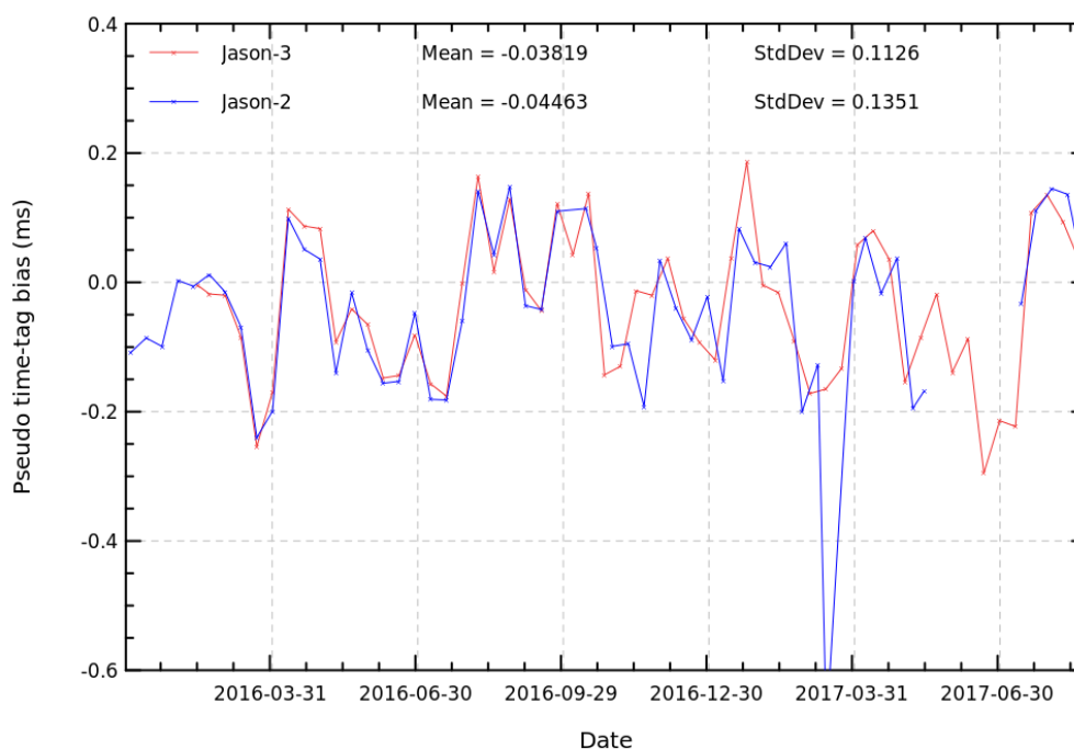
FIGURE 15 – Cyclic monitoring of pseudo time tag bias for Jason-3 and Jason-2.
