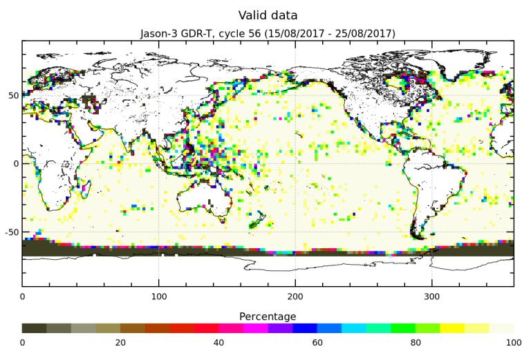
FIGURE 3 – Percentage of valid measurements for cycle 056.
