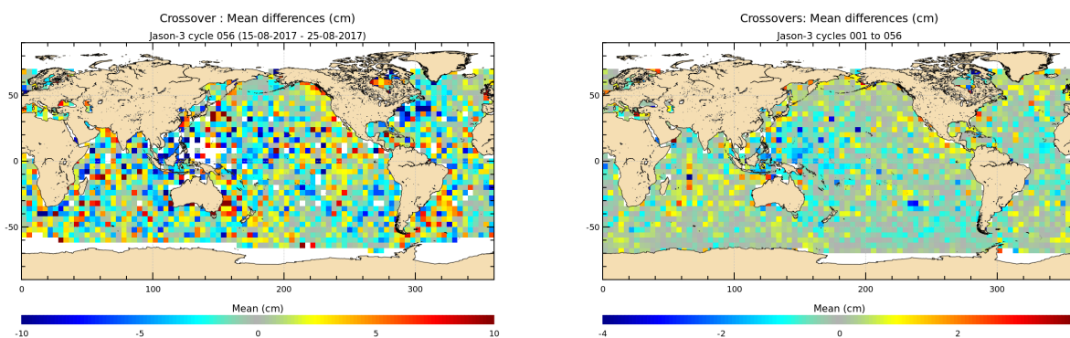
FIGURE 12 – Mean SSH at crossovers for cycle 056 (left) and over the whole Jason-3 period (right).
