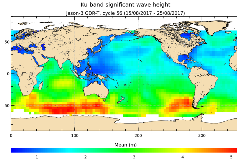
FIGURE 5 – Significant wave height for cycle 056.
