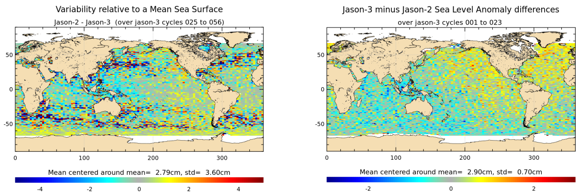
FIGURE 18 – Jason-2 – Jason-3 SLA differences averaged over Jason-3 period from cycle 025 until cycle 056 (left), and for tandem phase (cycle 001 to 023) (right).
