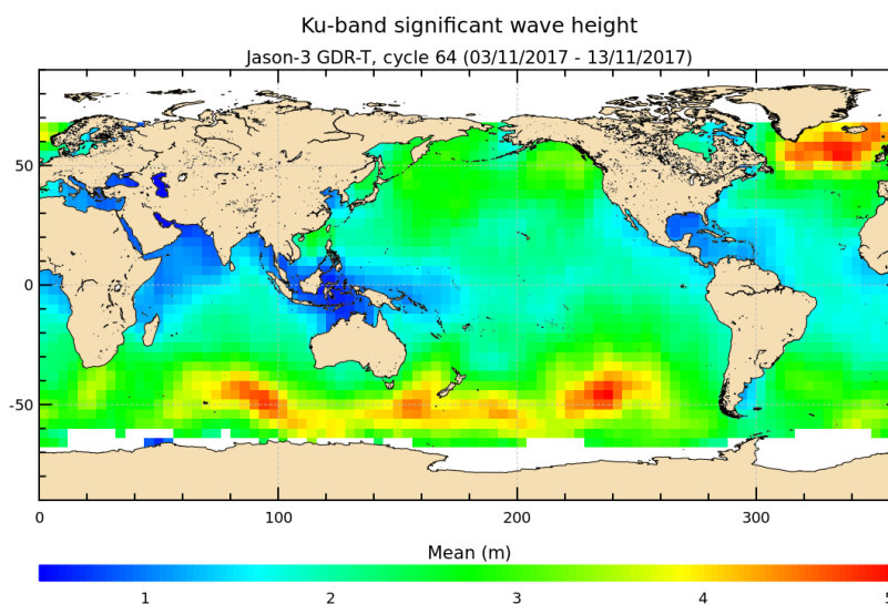
FIGURE 5 – Significant wave height for cycle 064.
