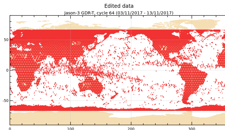
FIGURE 2 – Edited measurements for cycle 064.
