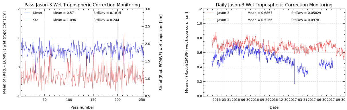
FIGURE 11 – Pass monitoring of wet troposphere differences between radiometer and ECMWF model for Jason-3 cycle 064 (left) and Jason-3 versus Jason-2 daily monitoring of wet troposphere differences between radiometer and ECMWF model (right).
