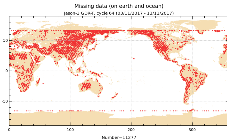
FIGURE 1 – Missing measurements for cycle 064.
