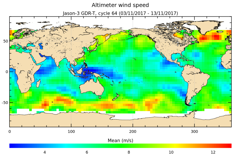
FIGURE 9 – Altimeter wind speed for cycle 064.
