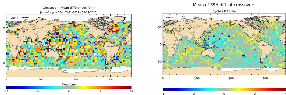
FIGURE 12 – Mean SSH at crossovers for cycle 064 (left) and over the whole Jason-3 period (right).
