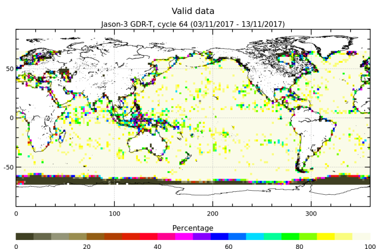
FIGURE 3 – Percentage of valid measurements for cycle 064.
