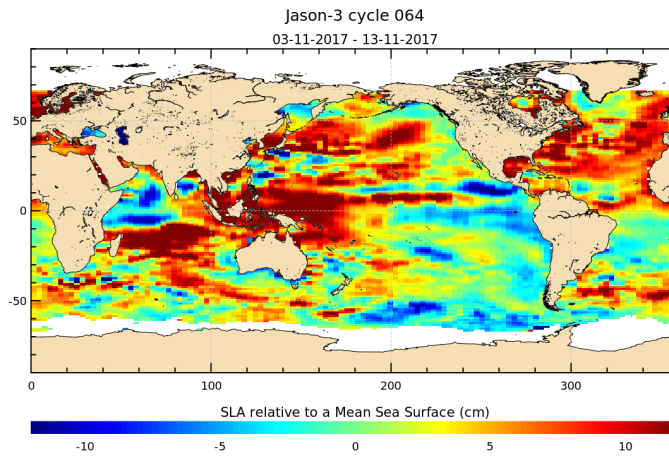
FIGURE 17 – Sea level anomaly relative to MSS for cycle 064.
