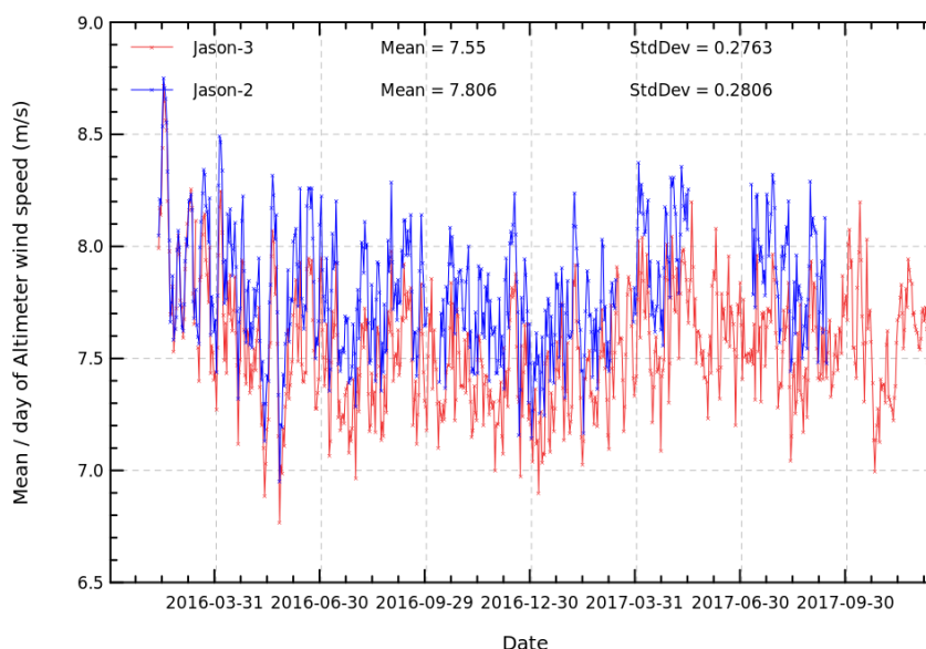
FIGURE 10 – Daily monitoring of altimeter wind speed for Jason-2 and Jason-3.
