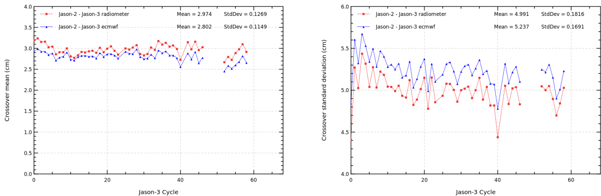
FIGURE 14 – Cyclic monitoring of mean (left) and standard deviation (right) of (Jason-2 – Jason-3) SSH differences at crossovers.
