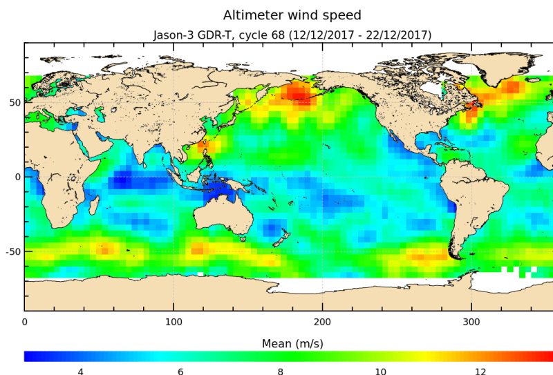
FIGURE 9 – Altimeter wind speed for cycle 068.
