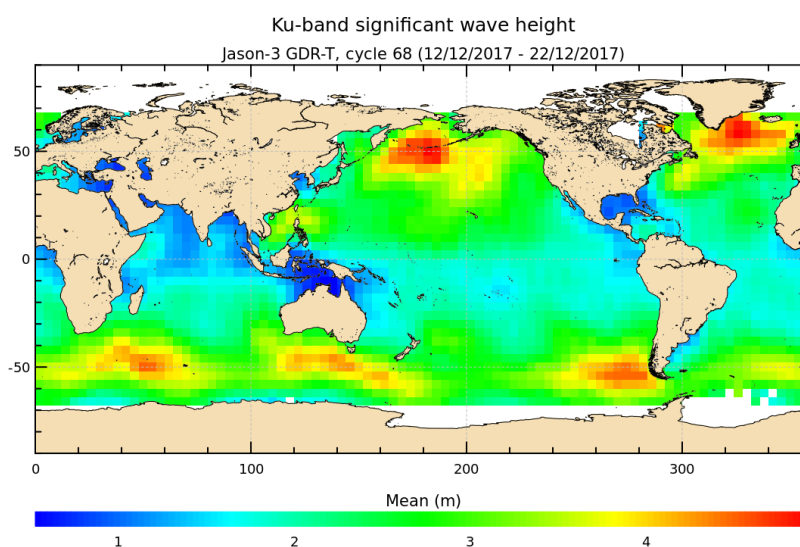
FIGURE 5 – Significant wave height for cycle 068.
