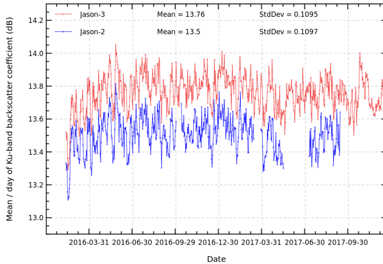
FIGURE 7 – Daily monitoring of Ku-band backscattering coefficient for Jason-2 and Jason-3.
