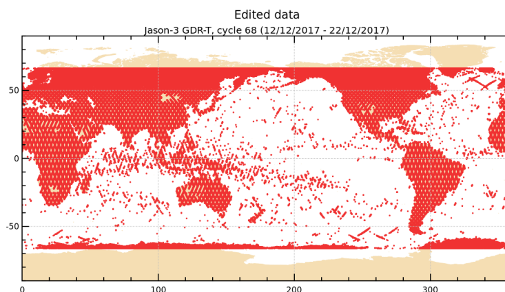
FIGURE 2 – Edited measurements for cycle 068.
