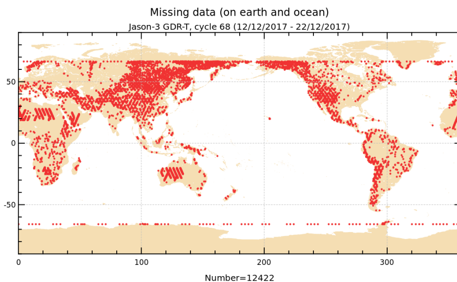
FIGURE 1 – Missing measurements for cycle 068.
