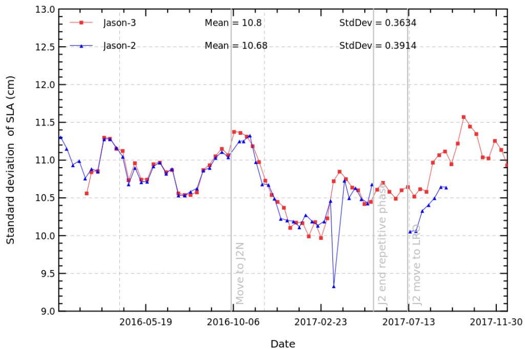
FIGURE 19 – Cyclic monitoring standard deviation of along track SLA for Jason-3 and Jason-2.
