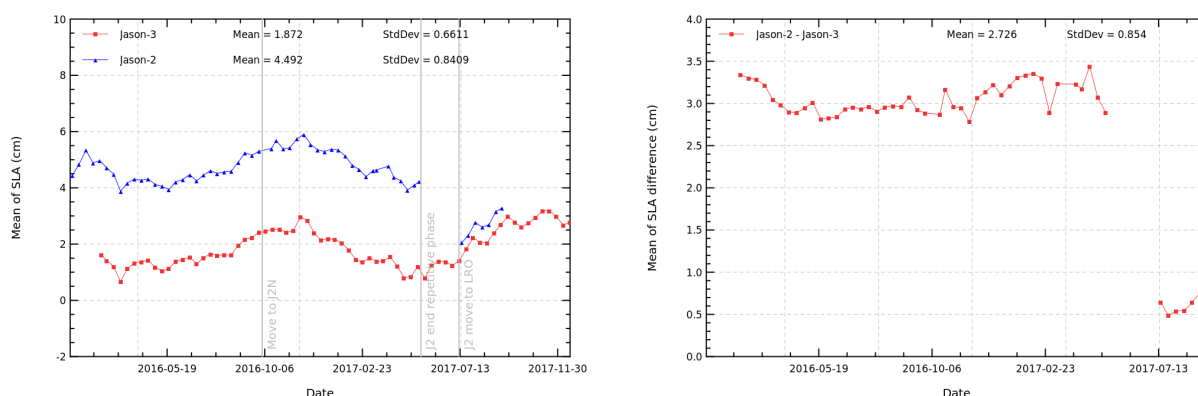
FIGURE 16 – Cyclic monitoring of mean SLA for Jason-3 and Jason-2 (left) and differences of (Jason-2 – Jason-3) mean SLA (right).
