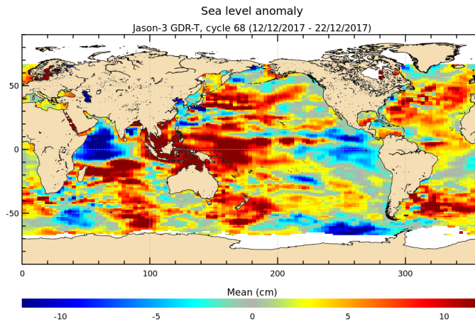
FIGURE 17 – Sea level anomaly relative to MSS for cycle 068.
