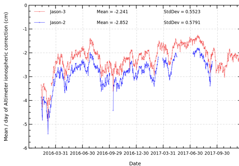
FIGURE 8 – Daily monitoring of dual-frequency ionosphere correction for Jason-2 and Jason-3.
