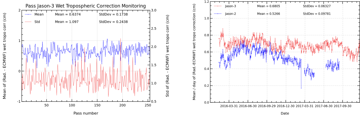
FIGURE 11 – Pass monitoring of wet troposphere differences between radiometer and ECMWF model for Jason-3 cycle 068 (left) and Jason-3 versus Jason-2 daily monitoring of wet troposphere differences between radiometer and ECMWF model (right).
