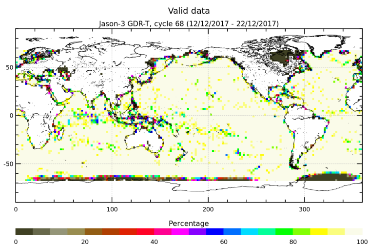
FIGURE 3 – Percentage of valid measurements for cycle 068.
