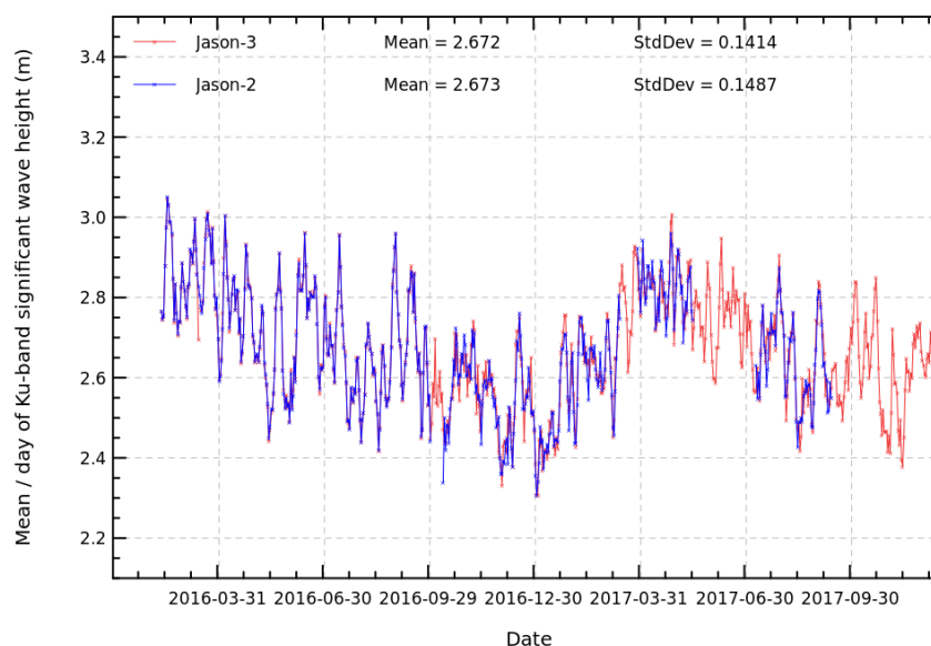
FIGURE 6 – Daily monitoring of Ku-band significant wave height for Jason-2 and Jason-3.
