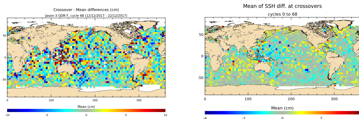
FIGURE 12 – Mean SSH at crossovers for cycle 068 (left) and over the whole Jason-3 period (right).
