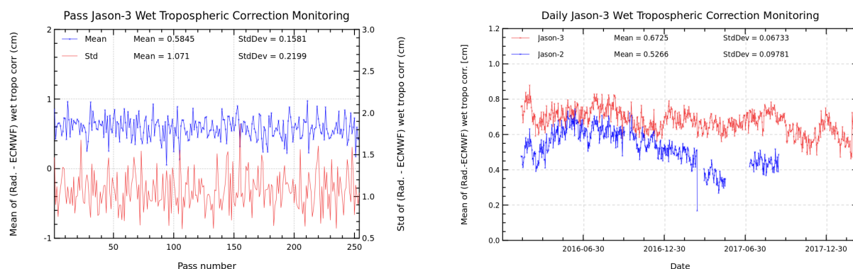
FIGURE 11 – Pass monitoring of wet troposphere differences between radiometer and ECMWF model for Jason-3 cycle 076 (left) and Jason-3 versus Jason-2 daily monitoring of wet troposphere differences between radiometer and ECMWF model (right).
