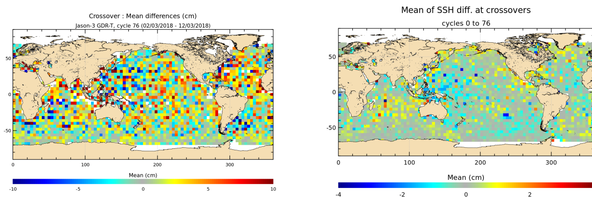
FIGURE 12 – Mean SSH at crossovers for cycle 076 (left) and over the whole Jason-3 period (right).
